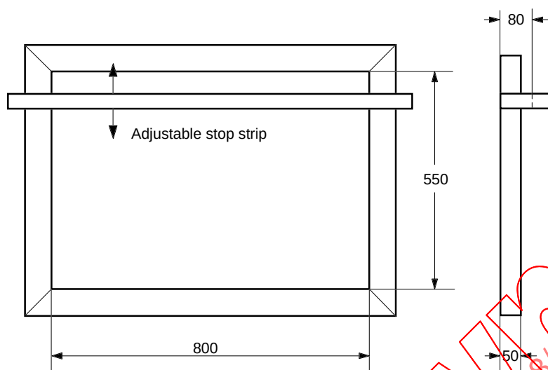
Figure 10B – Frame for test cushion
