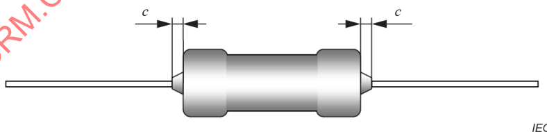
Figure 3 – Length of excessive coating on the wire terminations
