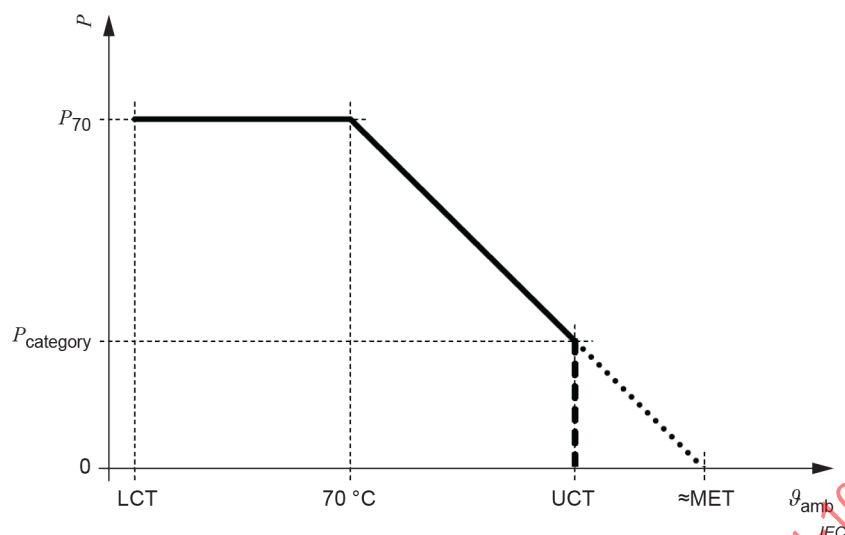
Figure 4 – Derating curve for power resistors
