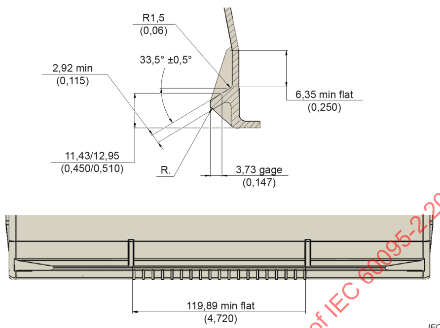
Figure 32 – Design for batteries with recesses on sides for hold-down-devices in mm and (in)
