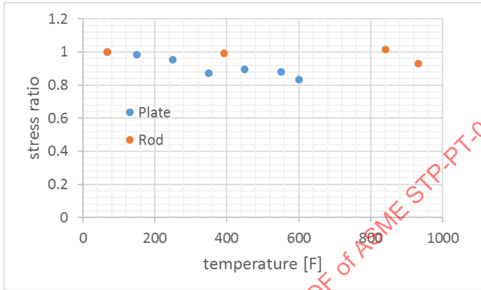
Figure 3-25: Comparison of available data for C70400
