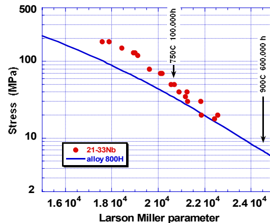
Figure 28 - Comparison of Alloy 21/33Nb Weld Strength with Alloy 800H Base Metal
