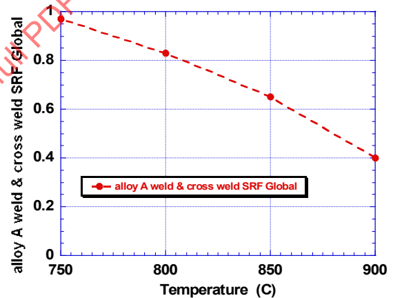
Figure 32 - Calculated Stress Rupture Factors for Alloy A for 100,000 hr.
