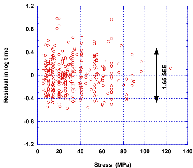
Figure 9 - Residuals vs. Stress for LM Parameter Fit to Alloy 800H
