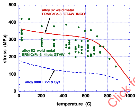
Figure 22 - Comparison of the Yield Strength for Alloy 82 Weld Metal with Alloy 800H
