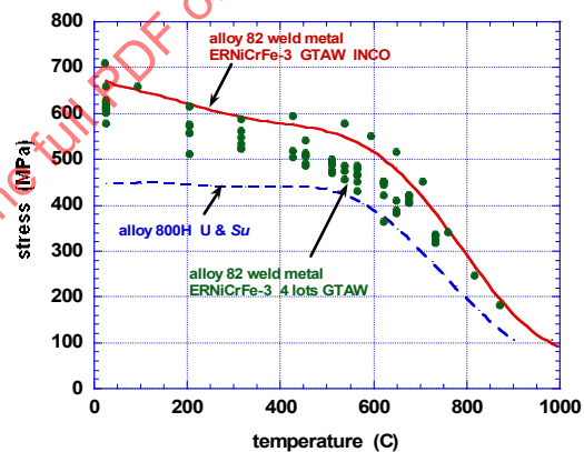
Figure 23 - Comparison of the Tensile Strength for Alloy 82 Weld Metal with Alloy 800H
