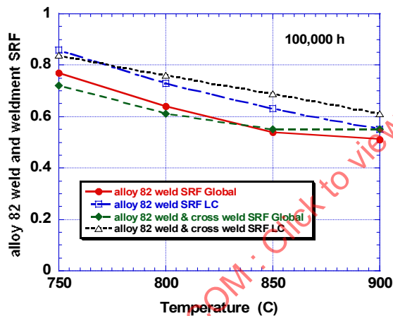
Figure 31 - Calculated Stress Rupture Factors for Alloy 82 for 100,000 hr.
