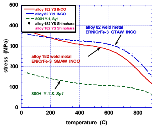
Figure 20 - Comparison of the Yield Strengths of SMA and GTA Weld Metals
