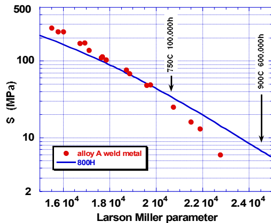
Figure 26 - Comparison of Alloy A Weld Strength with Alloy 800H Base Metal
