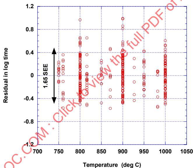
Figure 10 - Residuals vs. Temperature for LM Parameter Fit to Alloy 800H
