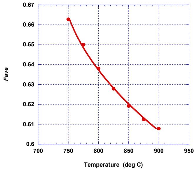
Figure 11 - F_{ave} vs. Temperature for Alloy 800H
