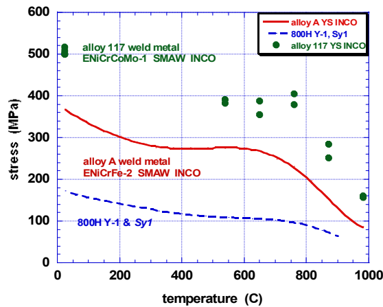
Figure 18 - Comparison of the Yield Strength for Alloy 117 Weld Metal with Alloy 800H
