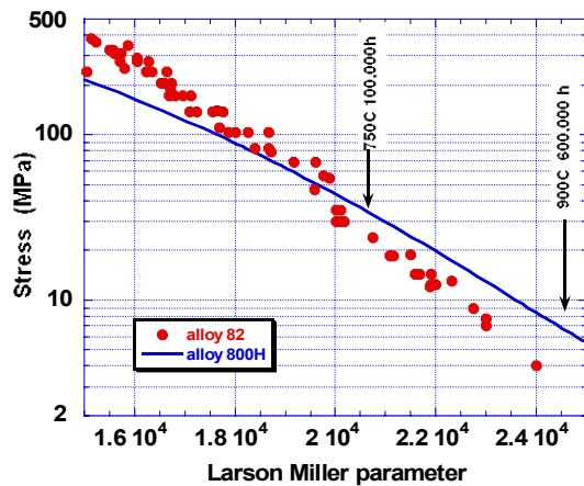
Figure 29 - Comparison of Alloy 82 Weld Strength with Alloy 800H Base Metal
