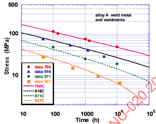
Figure 34 - Comparison of Rupture Data for Alloy A Weldments with Calculated Curves Based on the LMP
