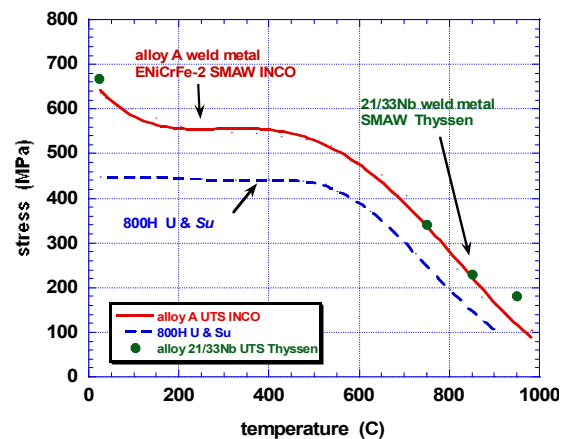
Figure 17 - Comparison of the Tensile Strength for 21/33Nb Weld Metal with Alloy 800H and Alloy A Weld Deposit
