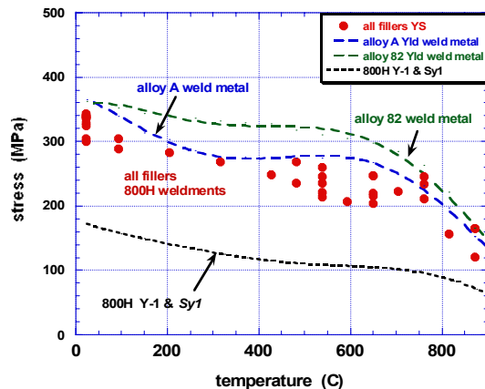
Figure 24 - Comparison of Weldment Yield Strength with Alloy 800H Base Metal
