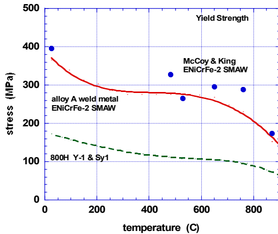
Figure 14 - Comparison of the Yield Strength for Alloy A Weld Metal with Alloy 800H
