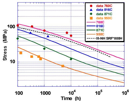
Figure 33 - Comparison of Rupture Data for Alloy 82 Weldments with Calculated Curves Based on the LMP
