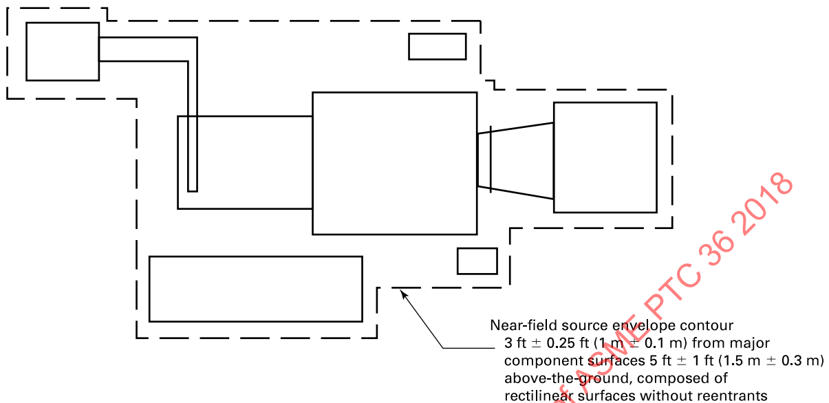
Figure 4-3.2.3-1 Near-Field Contours
