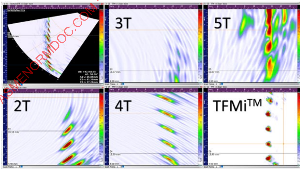
Figure 3-34: Sectorial scan, TFM images (2T-5T) and TFMi image for a sequence of side drilled holes vertically aligned.
