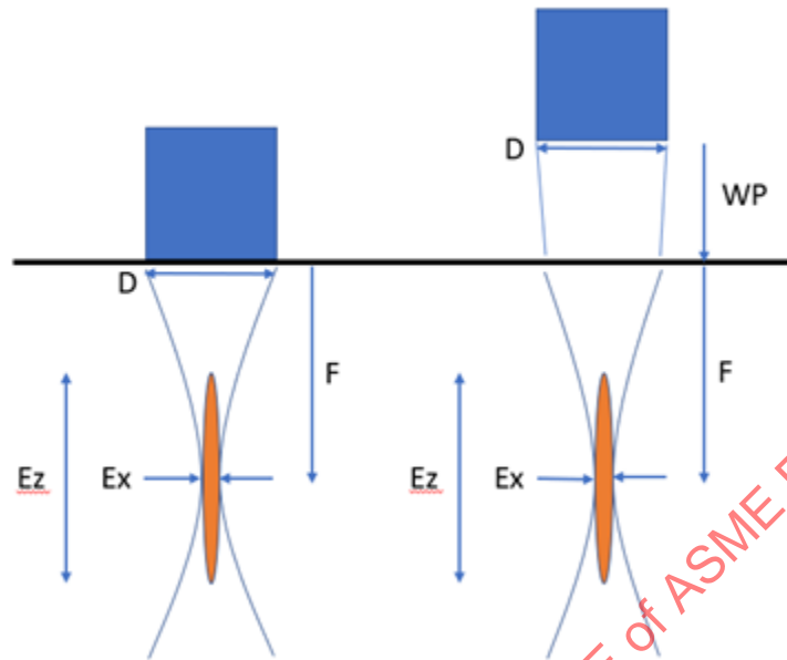
Figure 5-13: -6dB spot size (Ex) and -3dB depth of field (Ez) for flat and focused circular transducers
