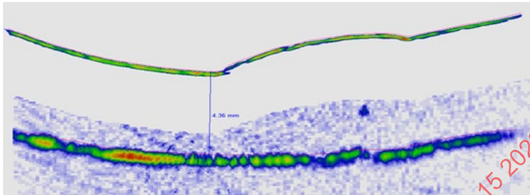
Figure 10-38: Minor inclusion from fabrication welding
