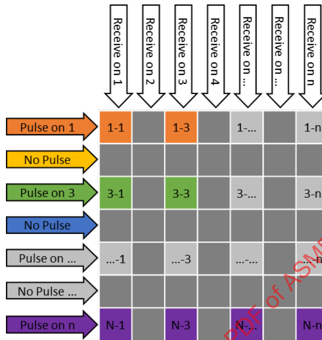
Figure 2-5: Example of a Possible SMC with 1:2 Sparsity
