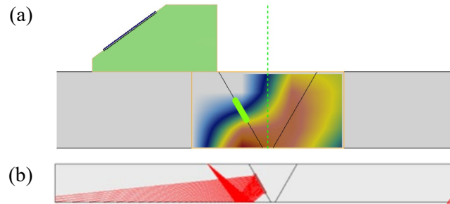
Figure 2-38: (a) Simulated acoustic field and (b) ray tracing results for a toe crack using TT-TT
