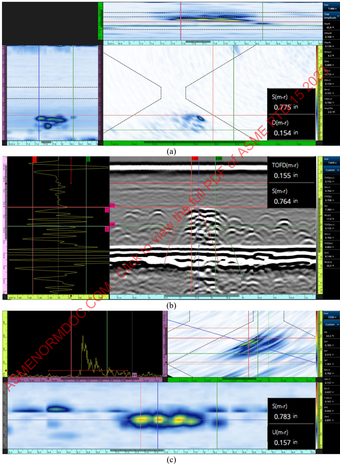
Figure 8-16: Images of Indication # 3 Porosity: (a) TFM T-T mode, (b) TOFD Non- Parallel Scan, (c) PAUT Sectorial Scan
