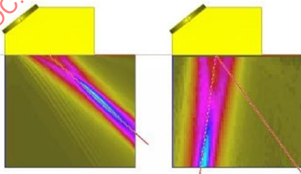
Figure 6-2: Fields radiated by the 45 T-wave transducer in isotropic (left) and anisotropic (right) specimens
