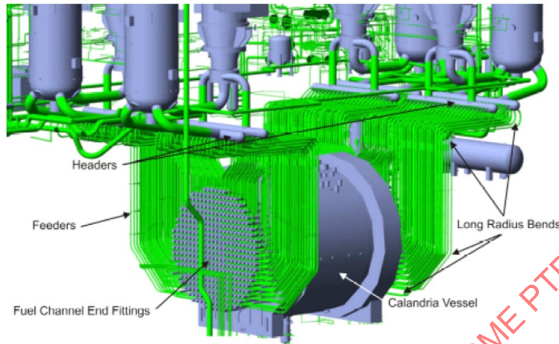
Figure 10-17: Primary Heat Transport piping arrangement between the steam generators and the fuel channels
