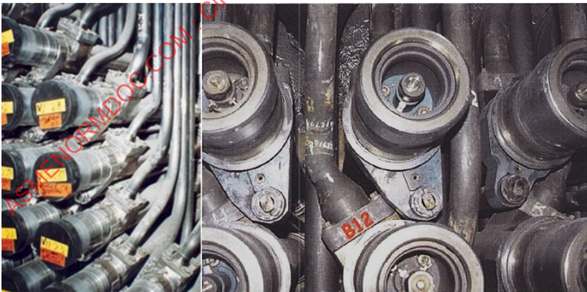
Figure 10-18: Example showing the typical congestion of the feeder pipes
