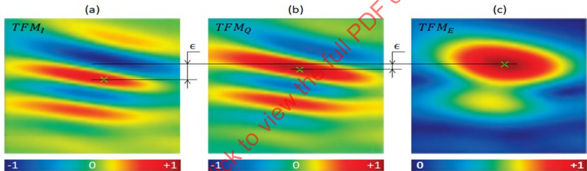
Figure 2-51: TFM images of a defect (SDH) showing a gap in the vertical position estimation of the maxima amplitude. (a) In-phase TFM–(b) Quadrature TFM–(c) Envelope TFM
