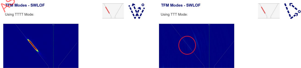
Figure 7-10: Lack of fusion detection comparison between TFM TT-TT and TT-T modes
