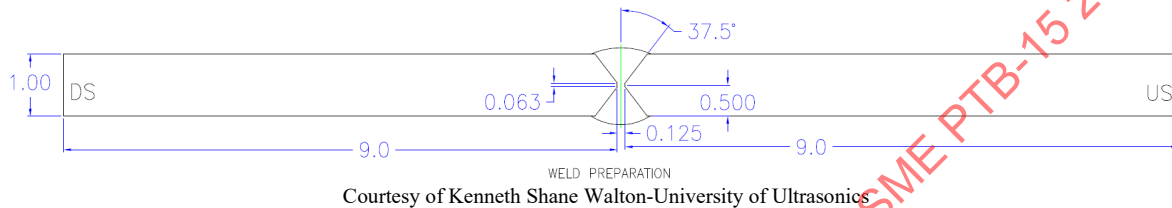
Figure 8-12: Weld Joint Geometry for 1 in. (25 mm) Samples
