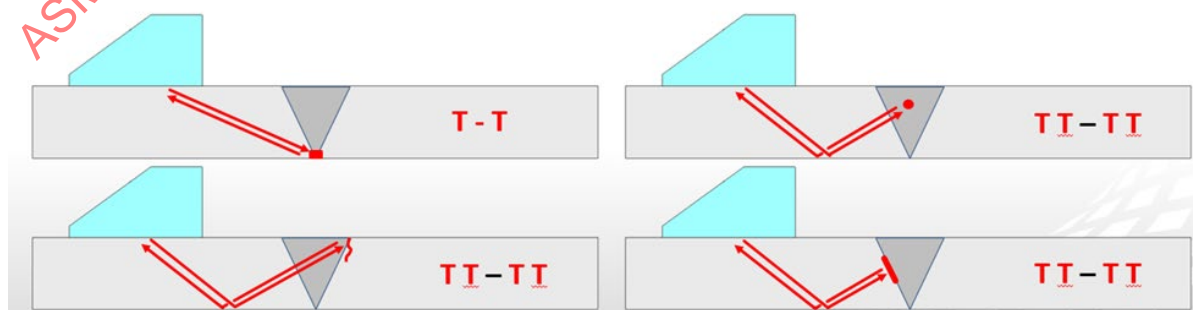
Figure 2-32: Acoustic paths and corresponding reconstruction modes for optimal detection of under evaluation flaws
