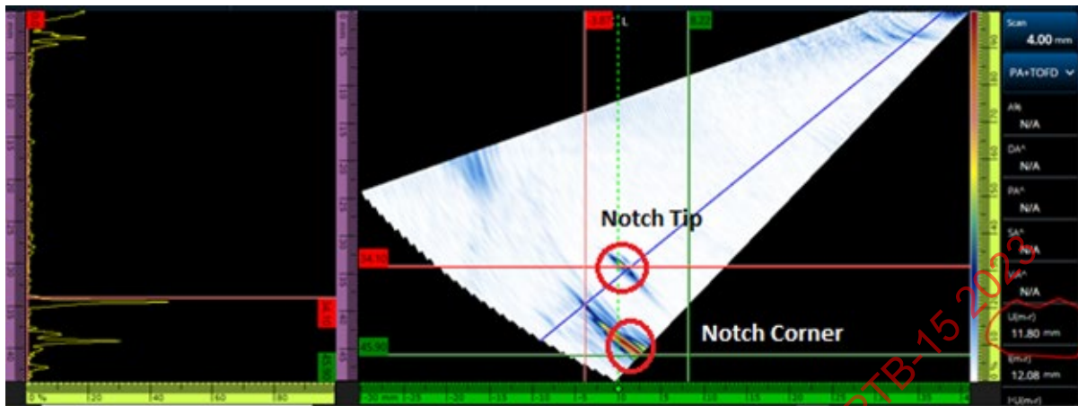
Figure 10-52: PAUT image (Sectorial Scan), Number of Cycles = 0
