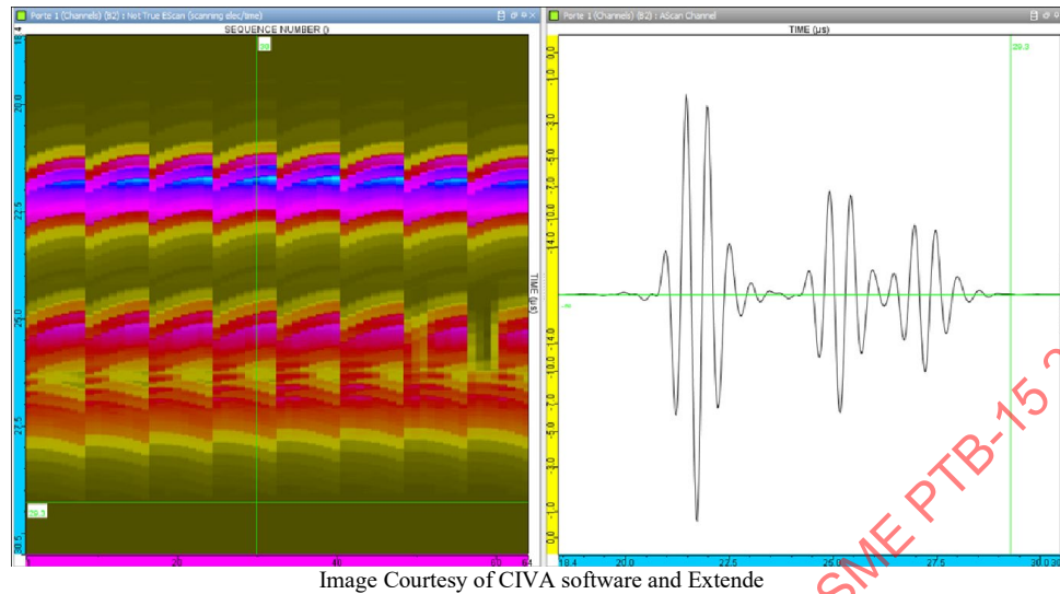
Figure 6-11: Raw results of the FMC simulation
