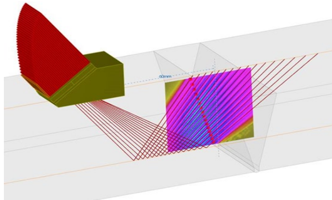
Figure 6-3: Beam of phased array transducer focused on weld prep
