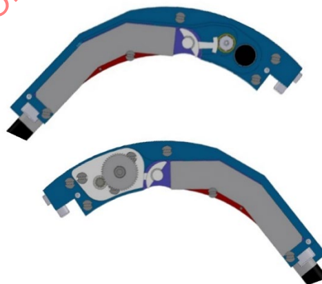
Figure 10-29: Manipulator arms
