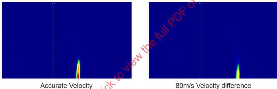
Figure 7-11: Vertical notch detection comparison with a TT-T mode of propagation: accurate velocity vs. 2.5% velocity input error
