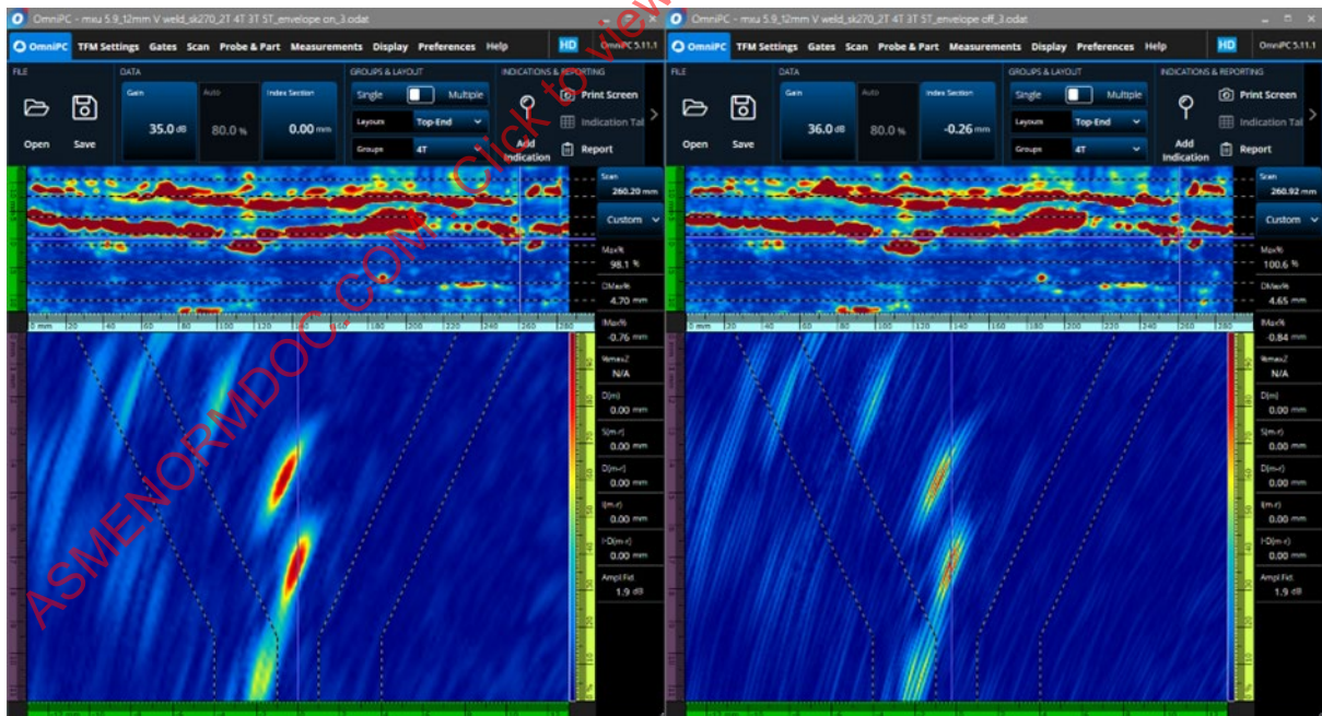
Figure 2-53: Examples of a slag indication. TFM image on the left with envelope and on the right without envelope.
