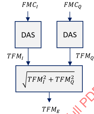
Figure 2-57: Computation of the envelope TFM from two FMCs in quadrature
