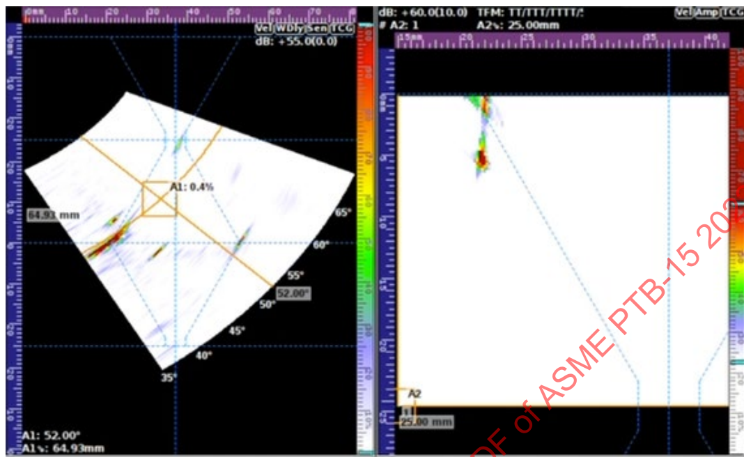
Figure 3-33: Toe crack. TFMi image on the right (2T-3T-4T) and sectorial scan on the left
