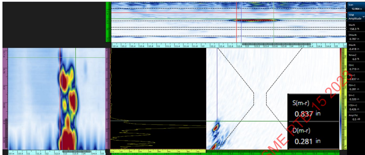
Figure 8-15: Images of Indication # 2-ID Crack: (a) TFM-T-T mode, (b) TOFD Non-Parallel Scan, (c) PAUT Sectorial Scan
