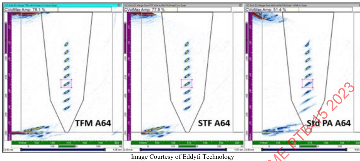
Figure 3-24: A comparison of TFM, STF, and standard PA
