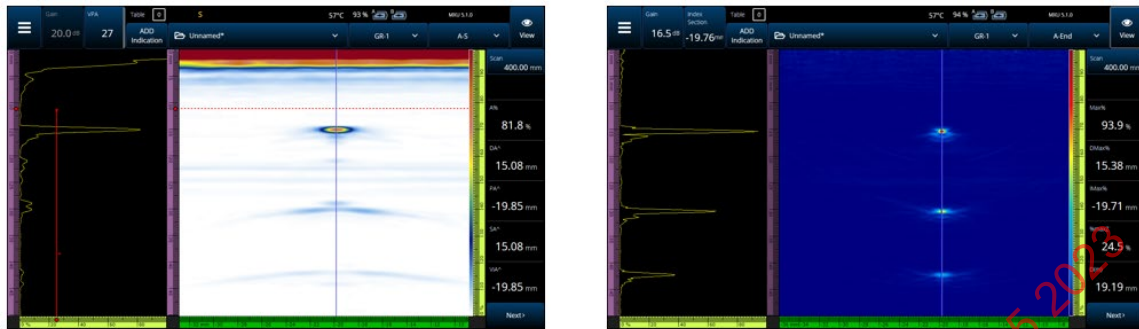
Figure 7-7: Detection of vertically stacked SDH comparison between PAUT and TFM L-L mode of propagation
