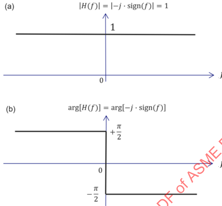
Figure 2-54: Transfer function of a Hilbert transform. (a) Modulus–(b) Phase
