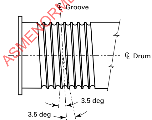
Fig. NUM-I-7942-1 Drum Fleet Angle
