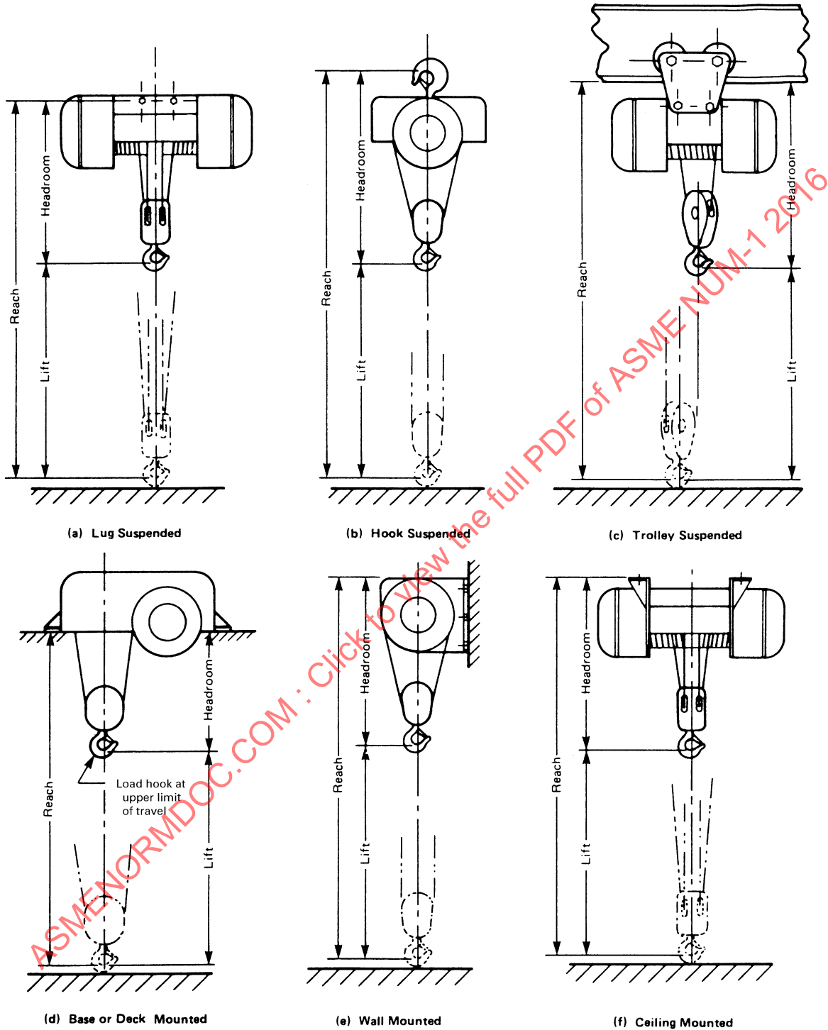
Fig. NUM-III-7210-1 Electric Wire-Rope Hoist, Suspension Types
