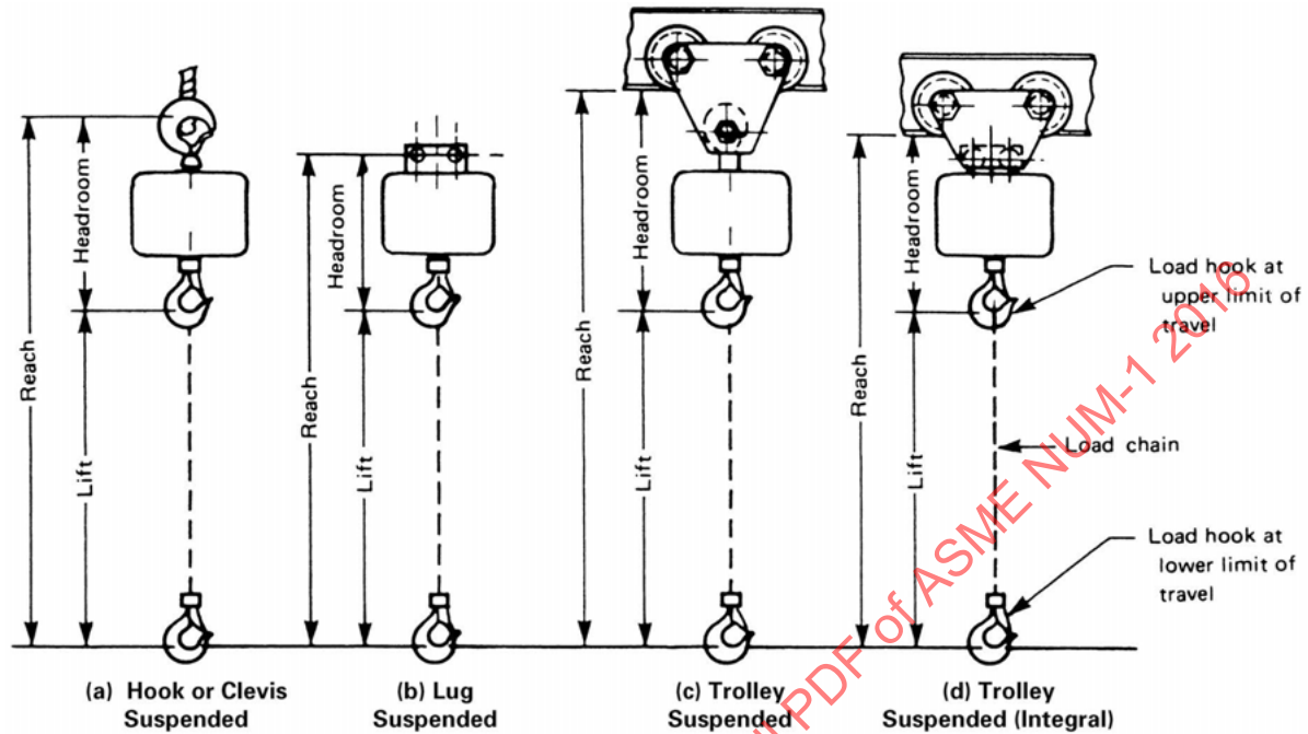
Fig. NUM-III-7610-1 Air-Operated Chain Hoist, Suspension Types
