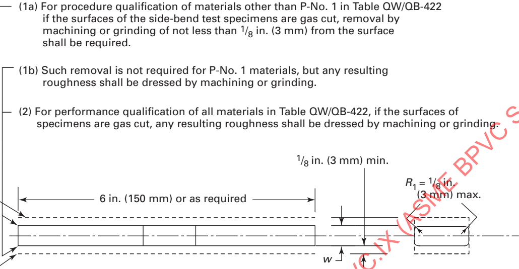
Figure QW-462.2 Side Bend
