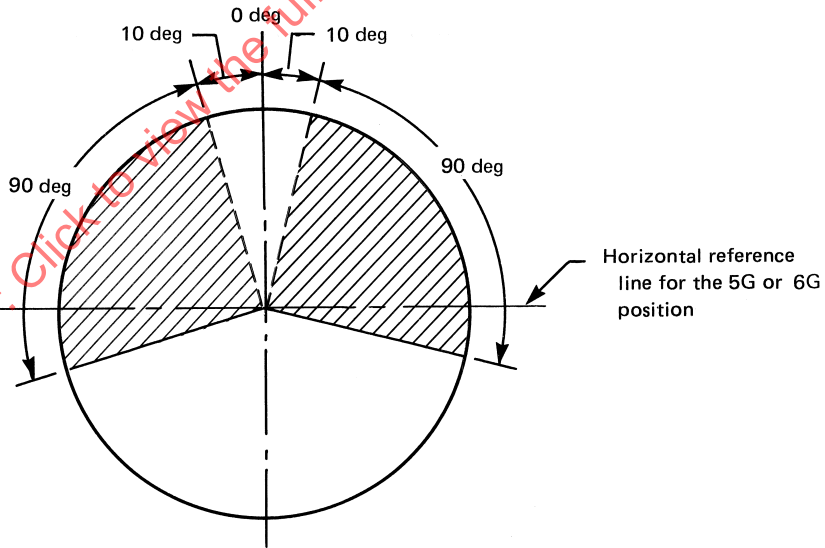
Figure QW-463.1(f) Toughness Test Specimen Location
