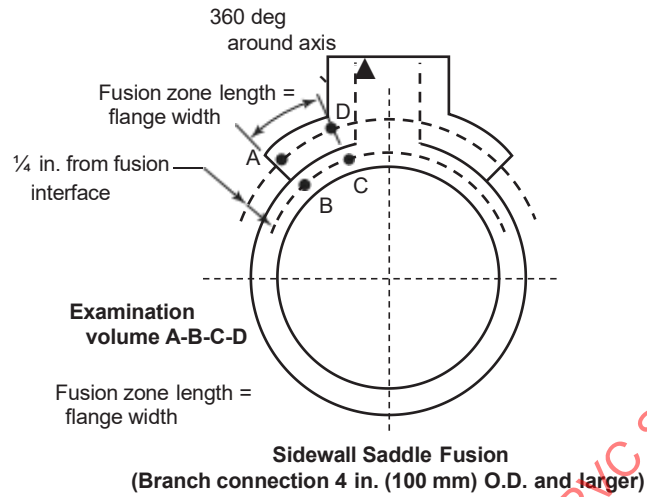
Figure XXVI-5220-3 Sidewall-Fusion Joint Examination Volume
