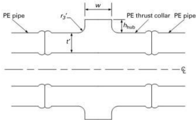
(c) Machined or Molded Polyethylene Thrust Collar
