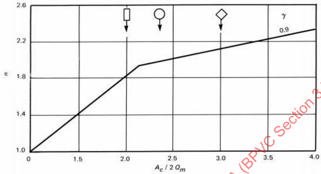
Figure A-9532(c)(3)-1 Interaction Exponent
