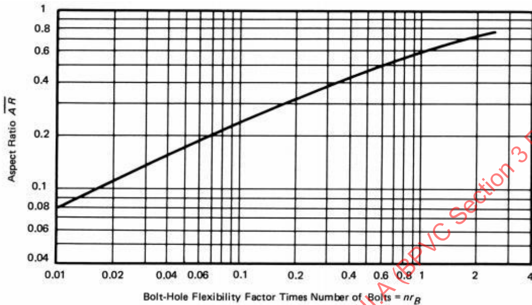
Figure L-3191-1 Bolt Hole Flexibility Factor
