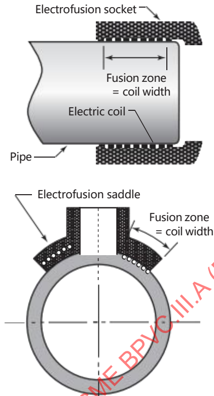
Figure XXVI-4110-2 Electrofusion Joint
