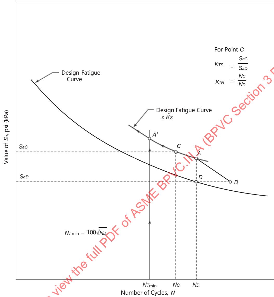
Figure II-1520(c)-2 Construction of the Testing Parameters Ratio Diagram for Accelerated Tests
