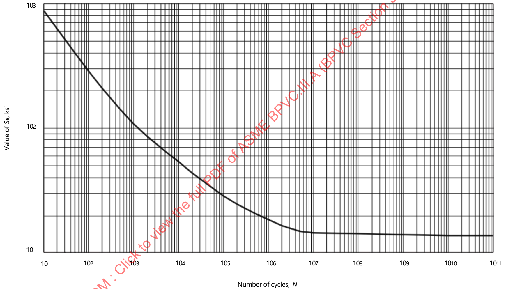
Figure I-9.2 Design Fatigue Curves for Austenitic Steels, Nickel-Chromium-Iron Alloy, Nickel-Iron-Chromium Alloy, and Nickel-Copper Alloy for Temperatures Not Exceeding 800°F
