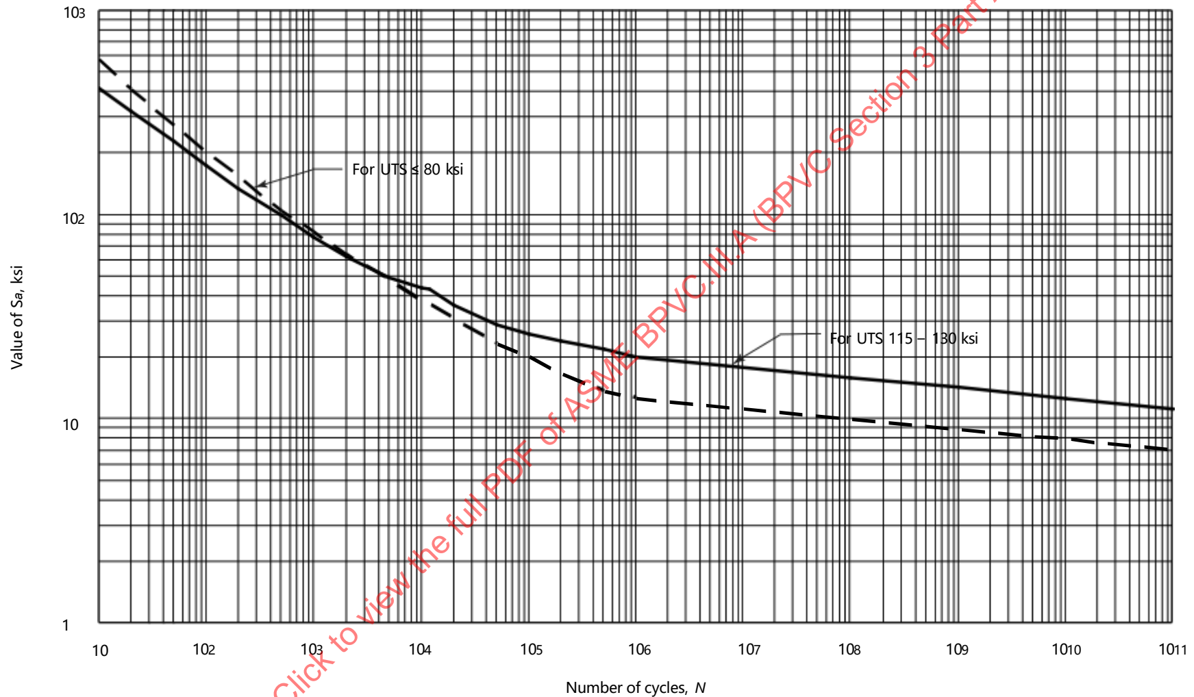
Figure I-9.1 Design Fatigue Curves for Carbon, Low Alloy, and High Tensile Steels for Metal Temperatures Not Exceeding 700°F
