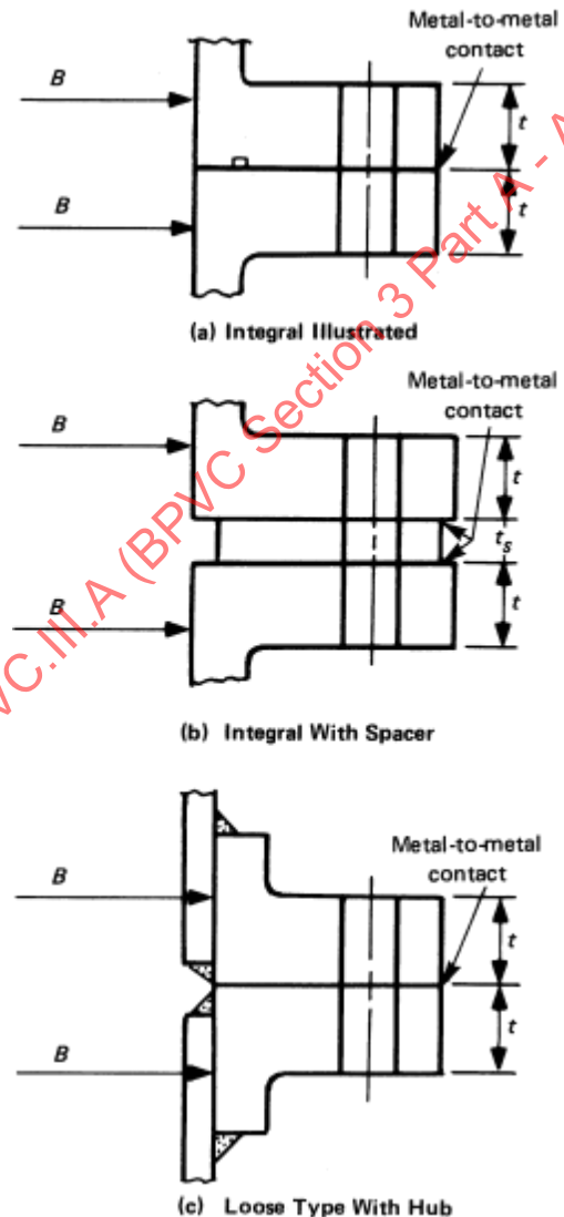
Figure L-3230-1 Group 1 Flange Assembly (Identical Flange Pairs)
