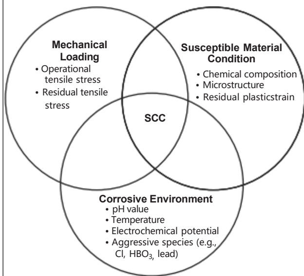
Figure W-2120-1 Environmental Conditions Required for SCC
