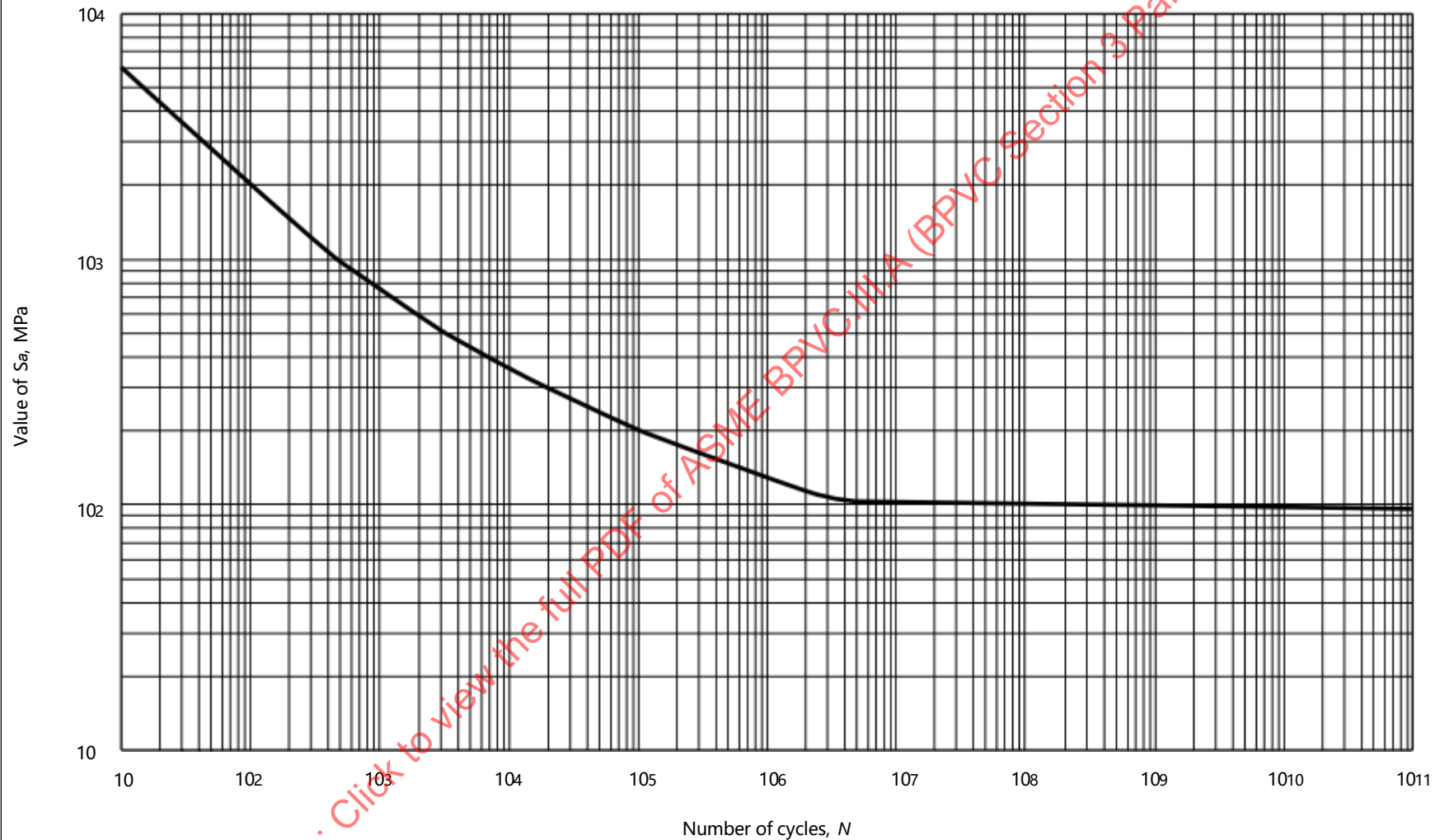
Figure I-9.2M Design Fatigue Curves for Austenitic Steels, Nickel-Chromium-Iron Alloy, Nickel-Iron-Chromium Alloy, and Nickel-Copper Alloy for Temperatures Not Exceeding 425°C
