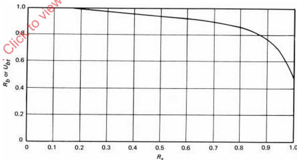
Figure A-9210(d)-1 Interaction Curve for Beams Subject to Bending and Shear or to Bending, Shear, and Direct Loads
