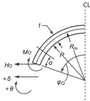
(a) Spherical Segment, for Values of \varphi_O : 162/\lambda \leq \varphi_O \leq 180 \text{ deg} - 162/\lambda
