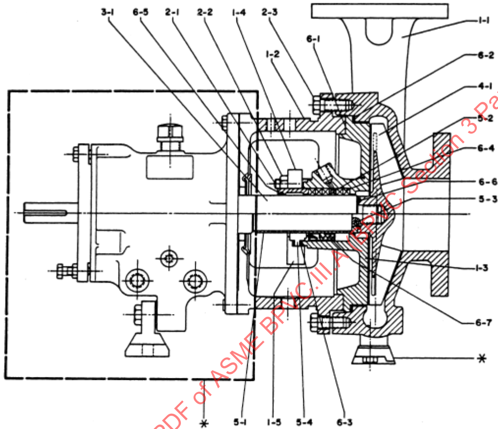
Figure U-1500-7 Typical for Type A and C Pumps (NCD-3400)
