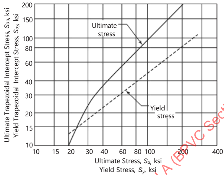
Figure A-9541-2 Ultimate and Yield Trapezoidal Intercept Stresses
