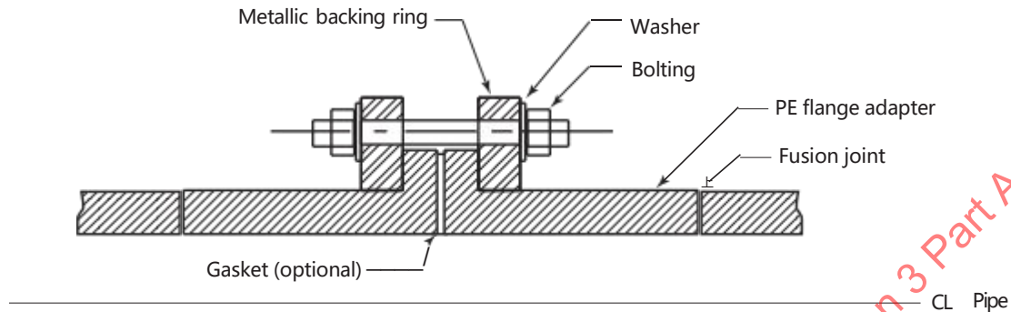
Figure XXVI-4520-2 Transition Flange Arrangement (HDPE to HDPE)
