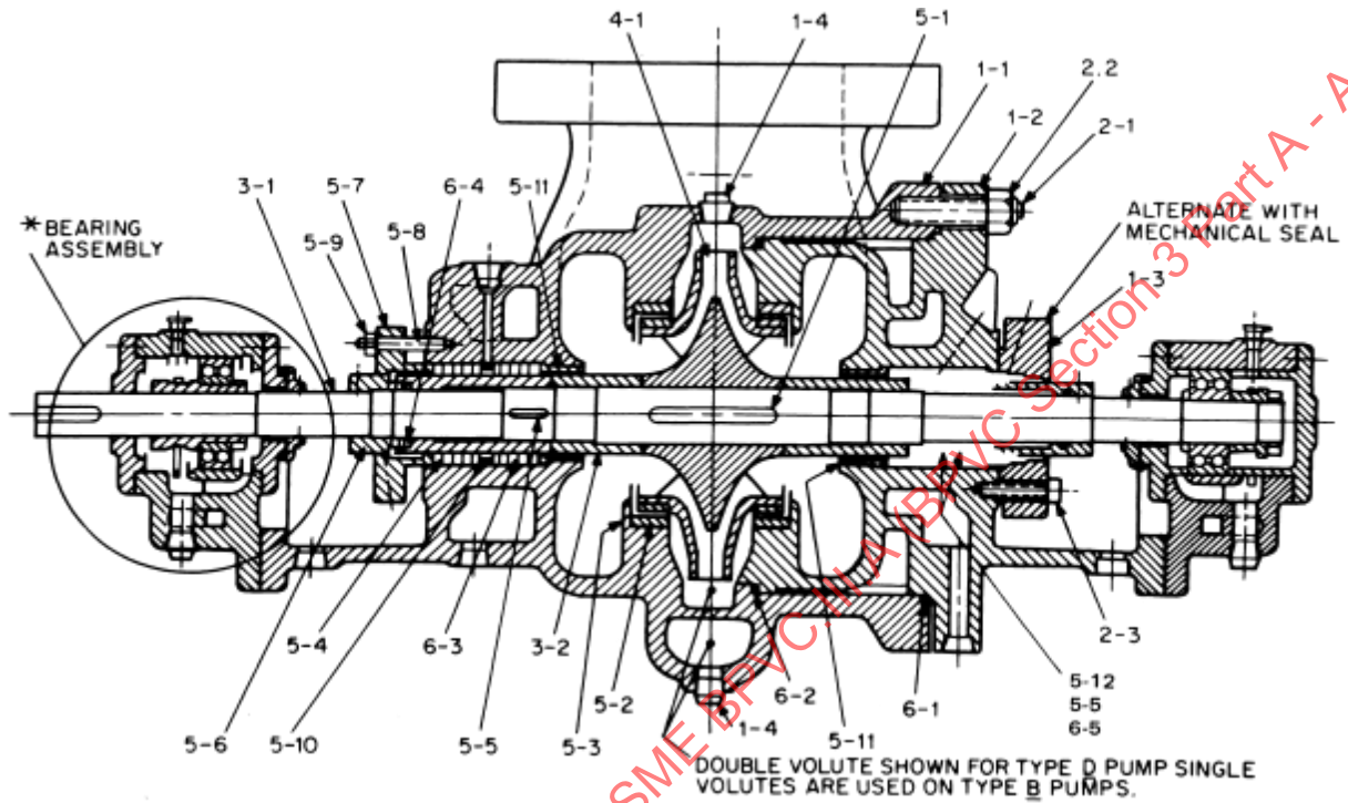
Figure U-1500-2 Typical for Type B and D Pumps (NCD-3400)
