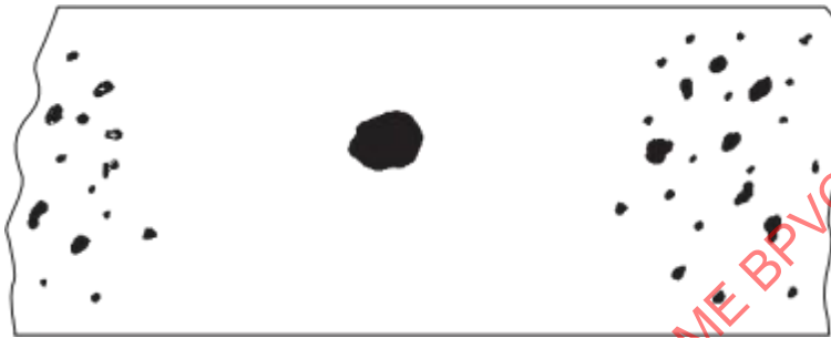
(a) Random Rounded Indications [Typical concentration and size permitted in any 6 in. (150 mm) length of weld.]
