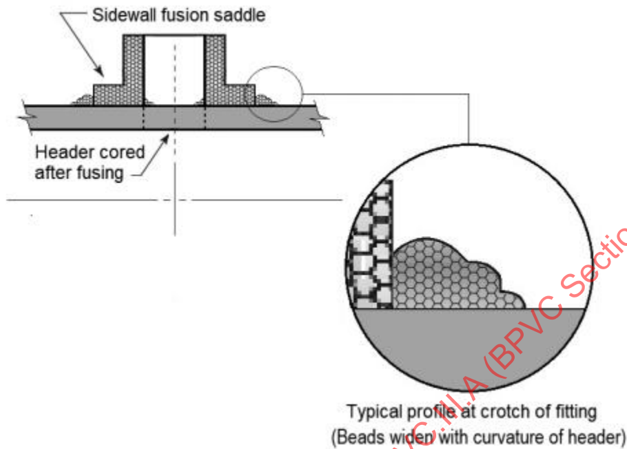
Figure XXVI-4110-3 Sidewall Fusion Joint
