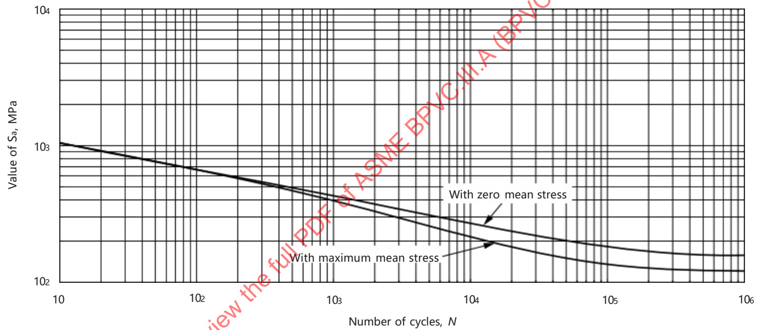
Figure I-9.6M Design Fatigue Curves for Grade 9 Titanium for Temperatures Not Exceeding 315°C
