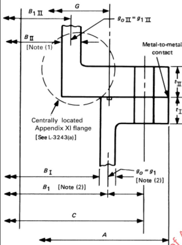
Figure L-3230-2 Group 2 Flange Assembly
