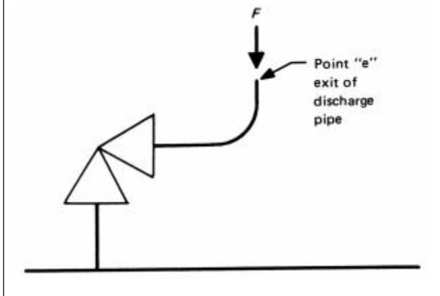
Figure O-1120(e)-1 Application Point of Venting Force F
