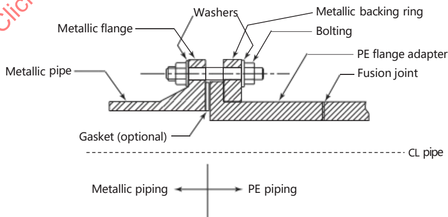
Figure XXVI-4520-1 Transition Flange Arrangement
