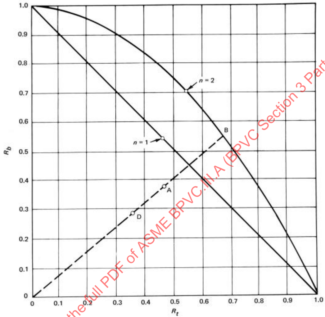
Figure A-9533(b)-1 Interaction Curve for Bending and Tension
