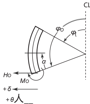
(c) Frustum, for Values of \varphi_O : \varphi_O \leq 180 \text{ deg} - 162/\lambda and |\varphi_O - \varphi| \geq 180/\lambda
