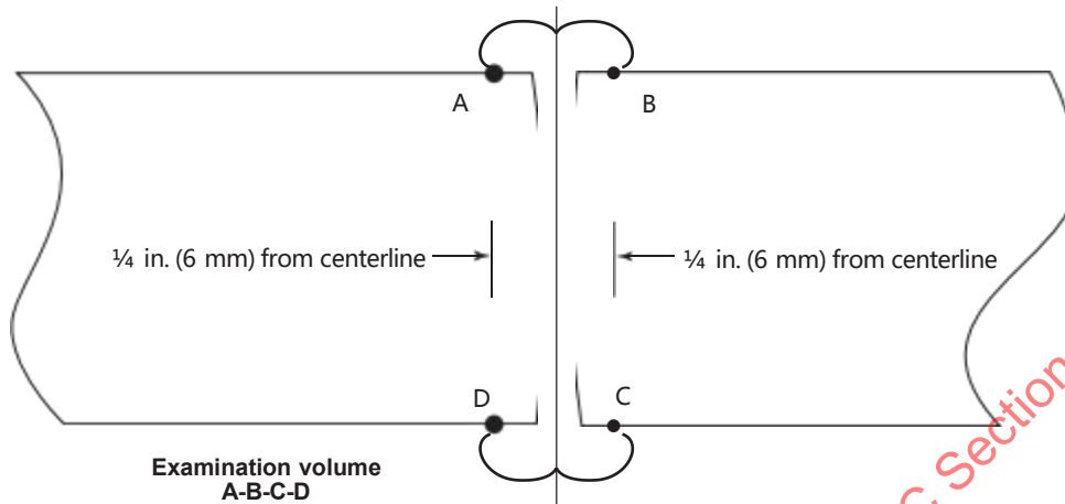
Figure XXVI-5220-1 Butt Fusion Pipe Joint Examination Volume
