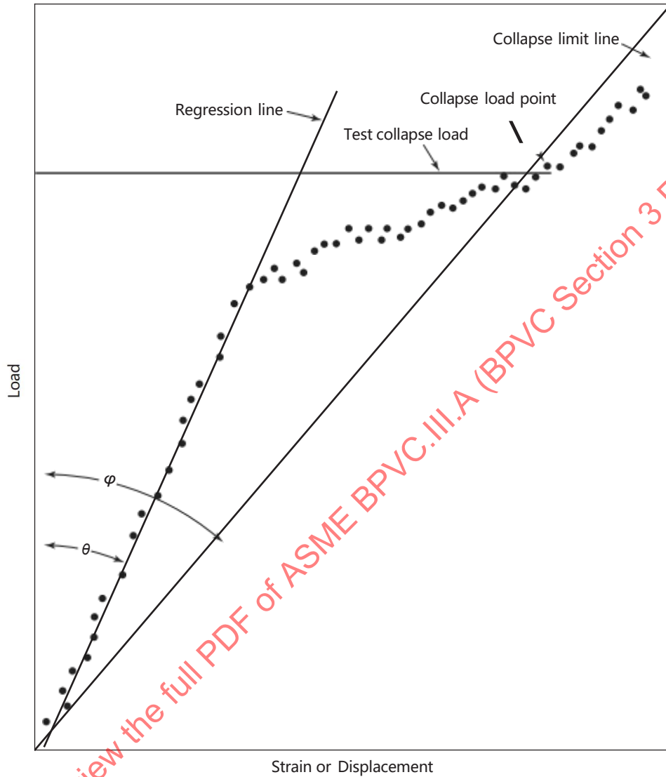
Figure II-1430-1 Construction for II-1430
