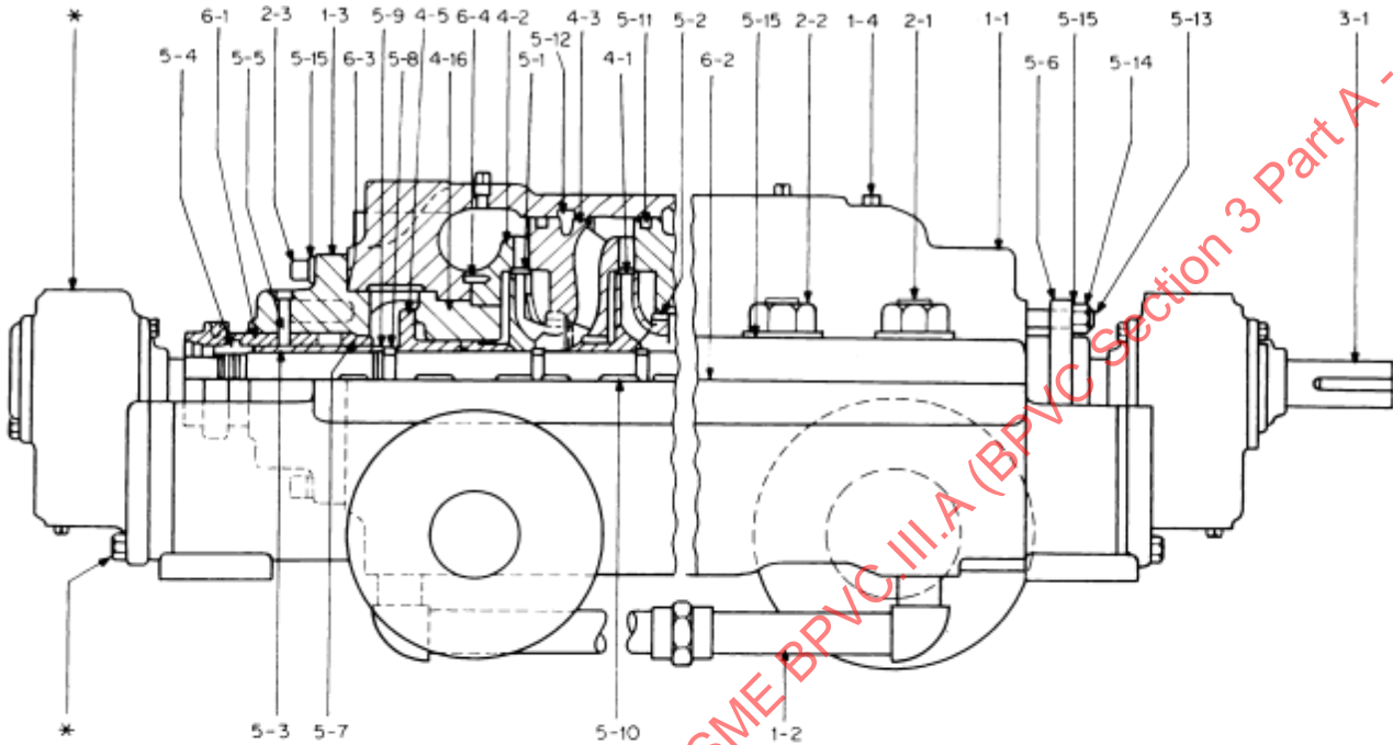
Figure U-1500-3 Typical for Type G and H Pumps (NCD-3400)
