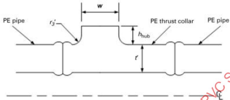
Figure XXVI-2234-1 Thrust Collars
