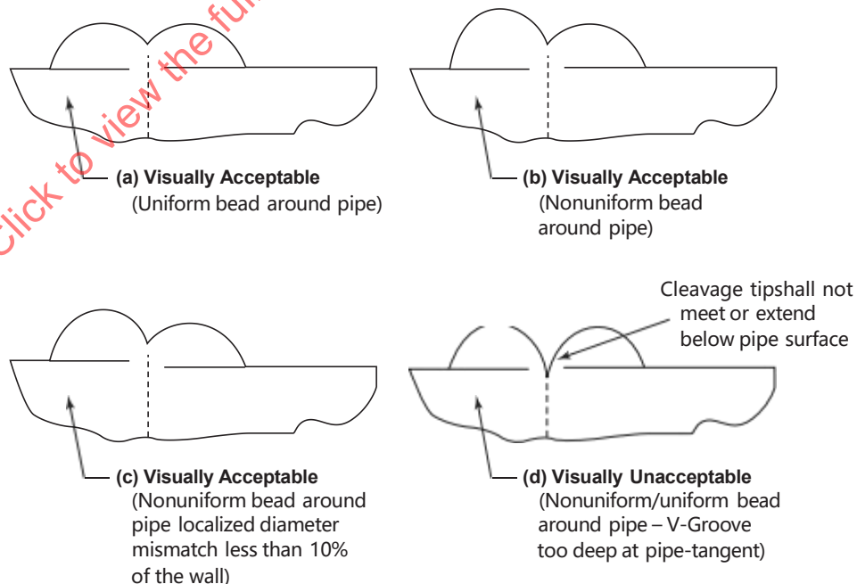
Figure XXVI-5321-1 Polyethylene Pipe Butt Fusion Joint O.D. Bead (Cross-Section View)
