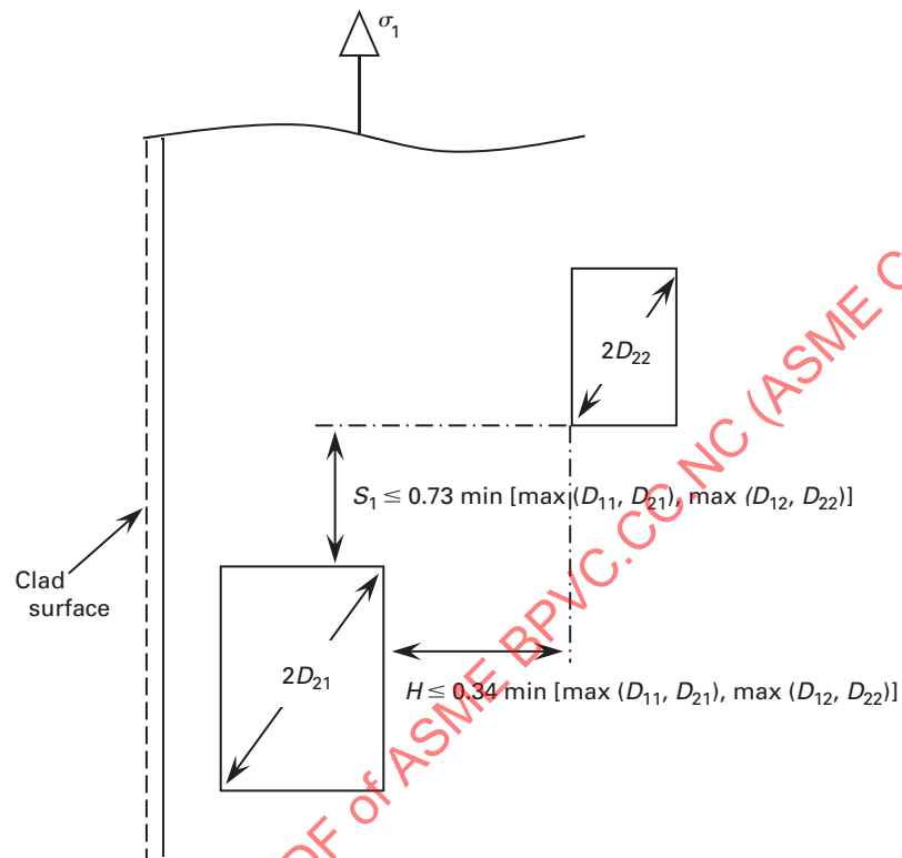
Figure 3 Proximity Rules for Multiple Quasi-Laminar Flaws
