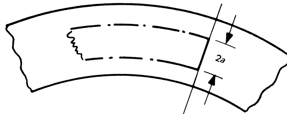
Figure A-2400-1 Flaw Characterization — Skewed Axial Flaws Projected into Axial Plane
