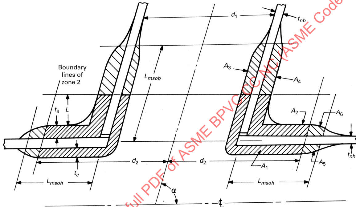
Figure -3643.3(c)-1 Reinforcement of Branch Connections
