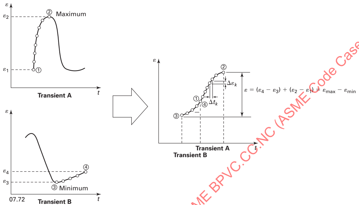
Figure -2600-1 Modified Strain Rate Calculation
