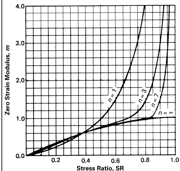
Figure -3742.6(h)-1 Zero Strain Modulus
