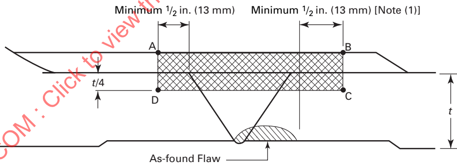
Figure 2(a) Examination Volume for Full Structural Weld Overlays
