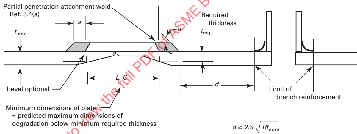
(a) Mitigation of Internal Corrosion
