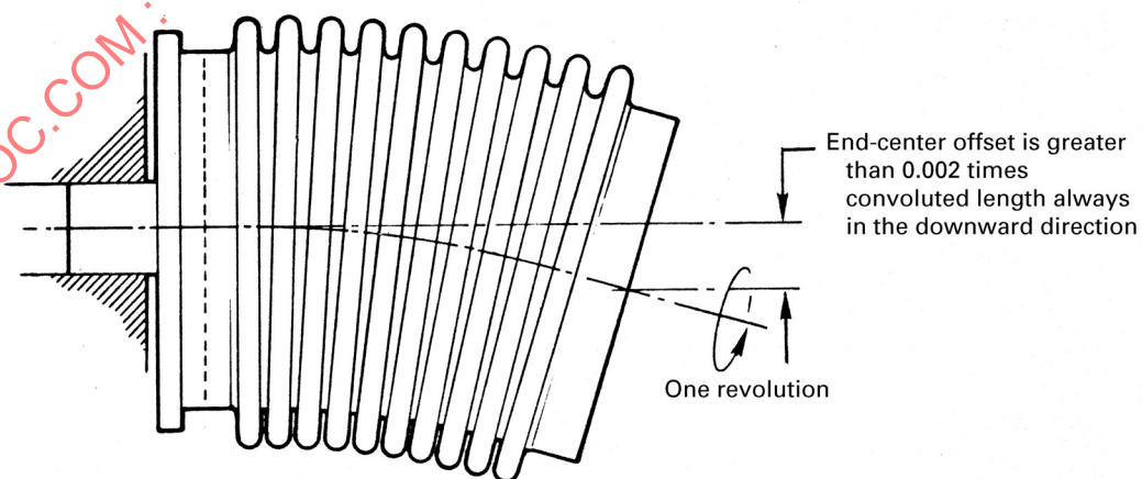
Figure -4224.1-3 Requirement for Proving Sufficient Flexibility to Allow Offset Fixturing
