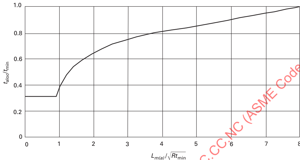
Figure 2 Allowable Wall Thickness and Length of Locally Thinned Area
