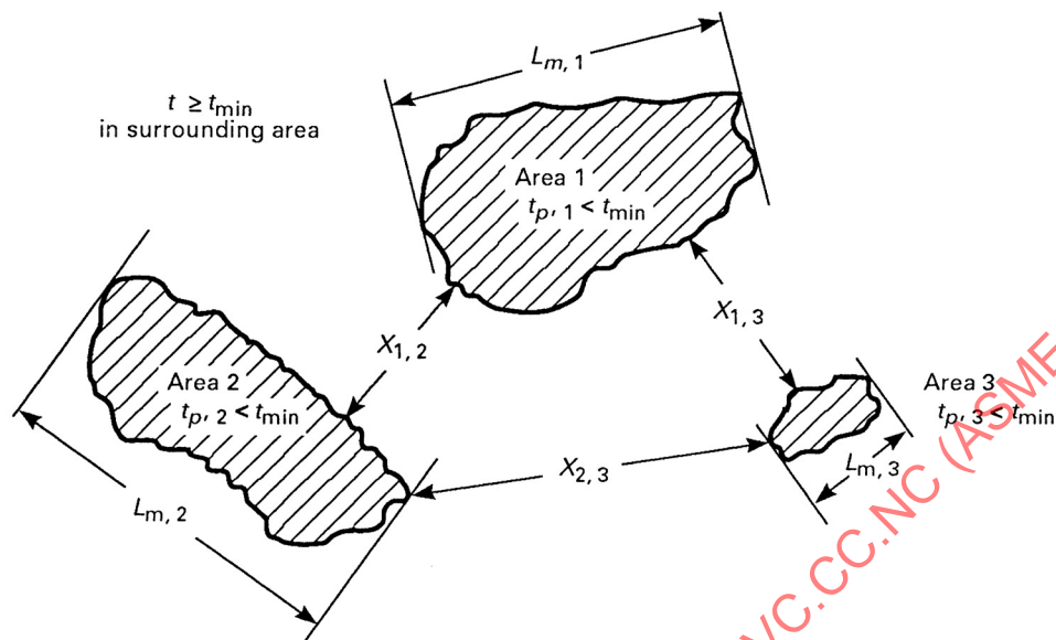
Figure 2 Separation Requirements for Adjacent Thinned Areas
