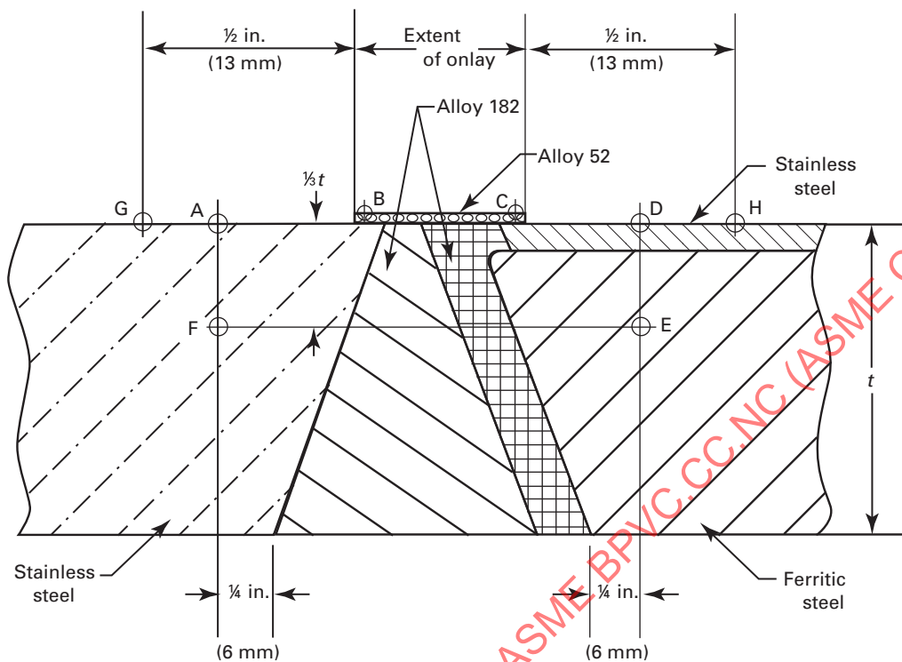
Figure 4 Examination Surface and Volume for Weld Inside Surface Onlay
