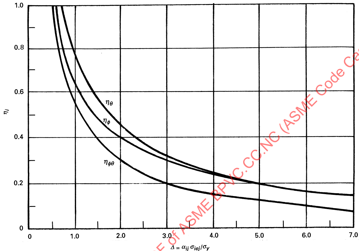
Figure -1610-1 Plastic Reduction Factors for Buckling Analysis by Formula
