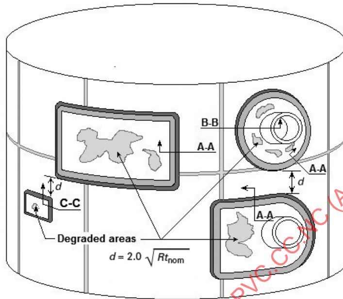
Figure 1 Shell Reinforcing Pads
