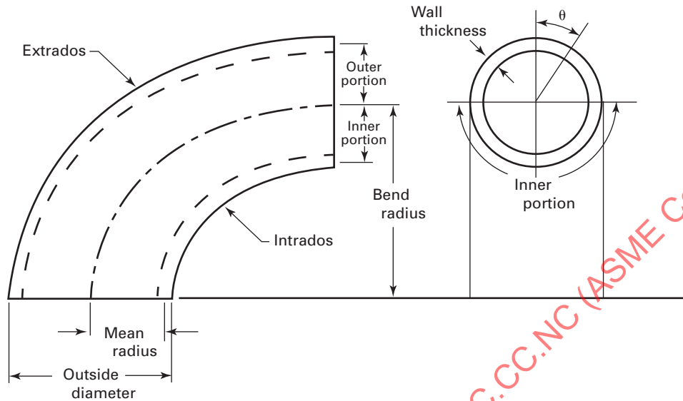
Figure -3622-4 Elbow or Pipe Bend
