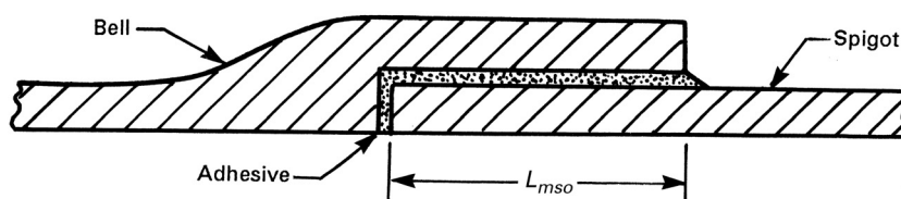
Figure -3662-1 Bell and Spigot Adhesive Bonded Joint
