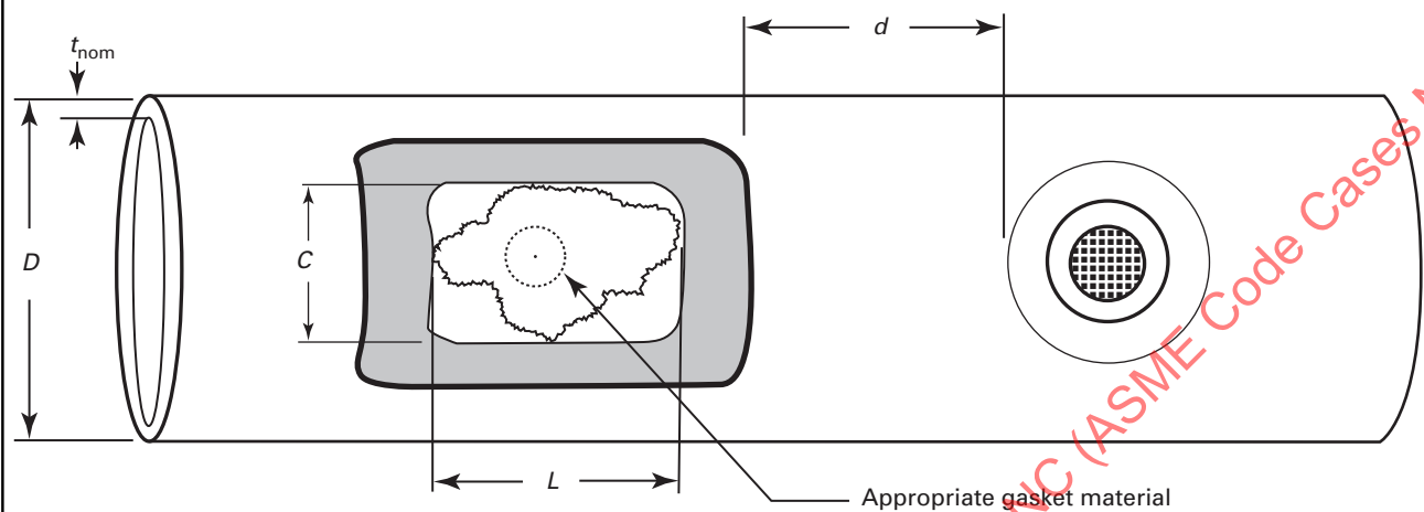
Figure 1 Structural Pad
