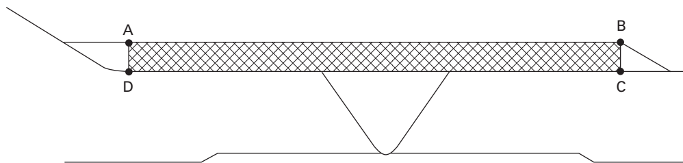
Figure 1 Acceptance Examination Volume and Thickness Definitions
