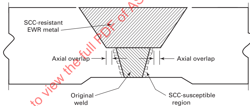
Figure 1B Cross Section of Typical Similar-Metal EWR
