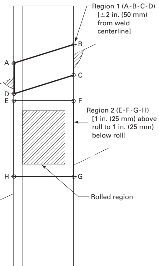
Figure 2 Examination Volume for BWR/6 CRD Housings
