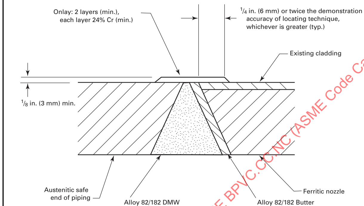
Figure 2 Typical Onlay
