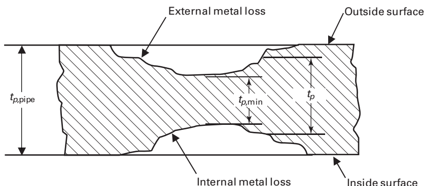
Figure 1 Illustration of Metal Loss Regions Due to Concurrent Internal and External Corrosion
