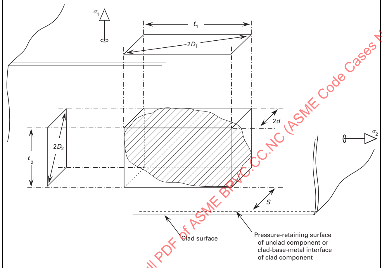
Figure 1 Configuration and Determination of Relevant Dimensions of a Quasi-Laminar Flaw
