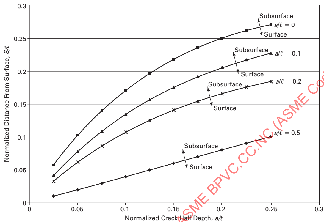
Figure 1 Successive Examination Surface Proximity Rule for Piping Components
