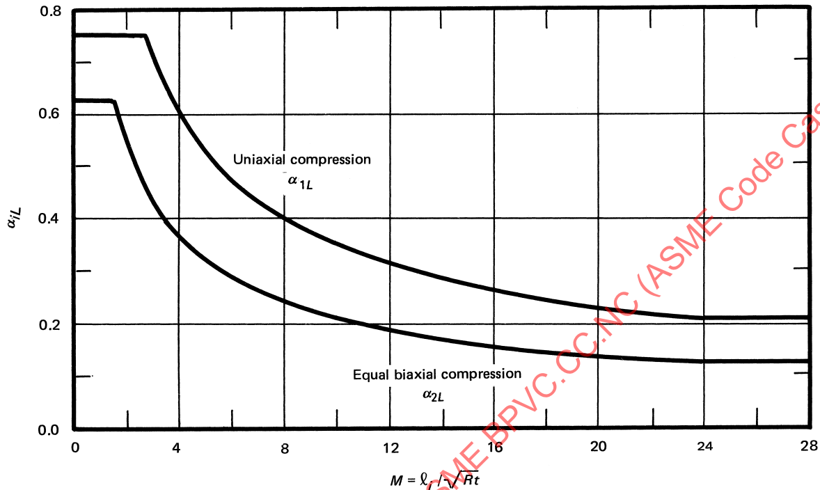
Figure -1512-1 Capacity Reduction Factors for Local Buckling of Stiffened and Unstiffened Spherical Shells
