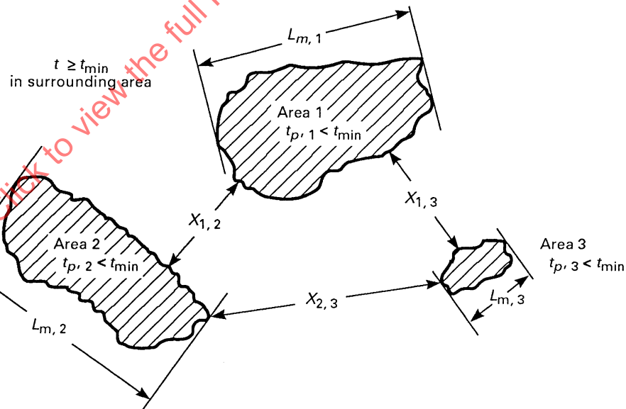
Figure -3622-5 Separation Requirements for Adjacent Thinned Areas With Limited Circumferential Extent (Hoop Stress Check)
