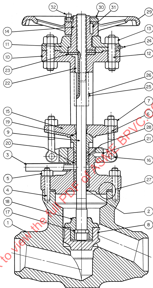
Figure 2 Globe Valve
