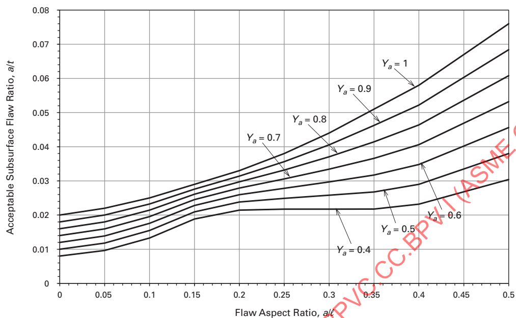
Figure 2 Alternative Subsurface Flaw Acceptance Criteria
