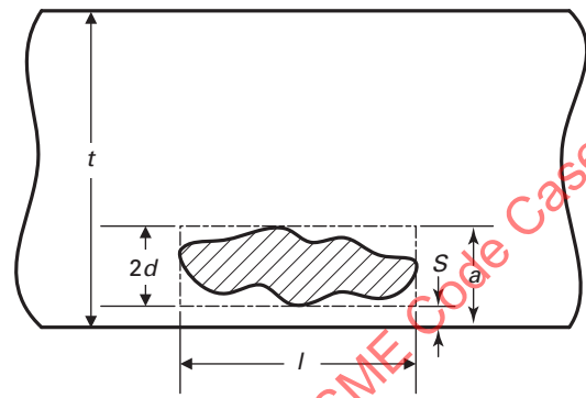
Figure 1 Alternative Flaw Classification of Single Indication
