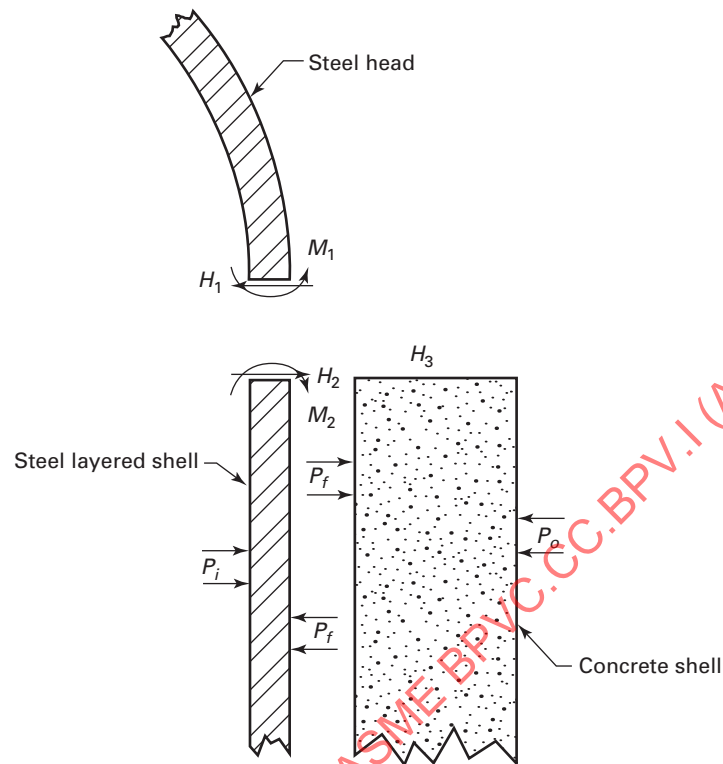
Figure 12 Head-to-Shell Forces
