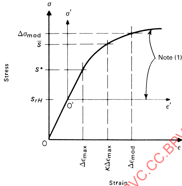
Figure 10 Stress-Strain Relationship
