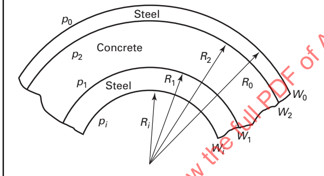
Figure 8 Steel-Concrete-Steel Interaction
