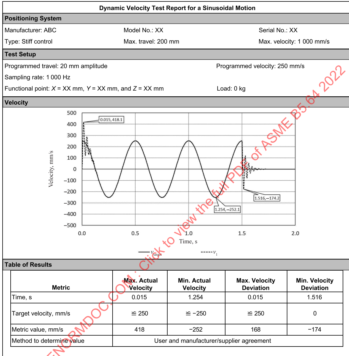
Figure 7-7.2-2 Example of a Dynamic Velocity Test Report for a Sinusoidal Motion
