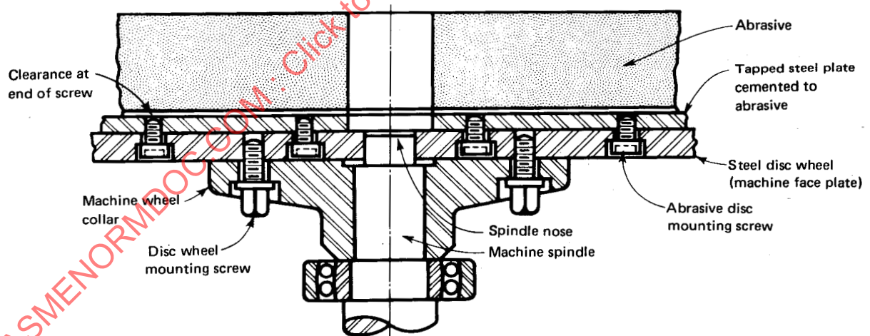
FIG. 3 TYPICAL TAPPED MOUNTING PLATE TYPE MOUNTING
