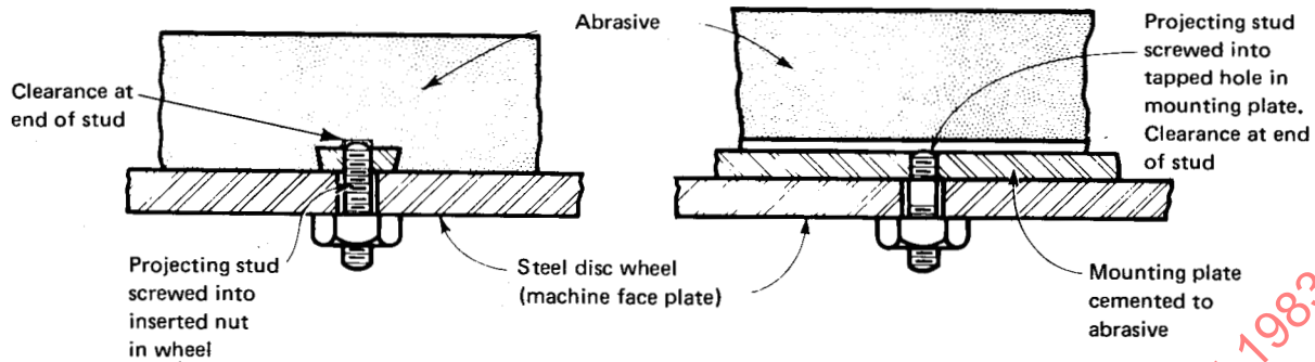
FIG. 4 TYPICAL PROJECTING STUD TYPE MOUNTINGS
