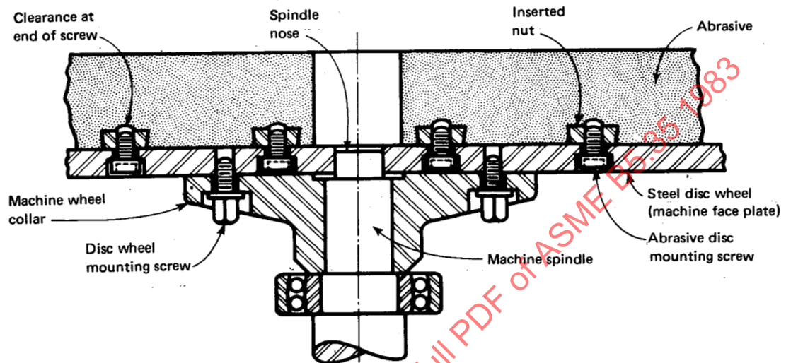
FIG. 1.1 TYPICAL INSERTED NUT TYPE MOUNTING
