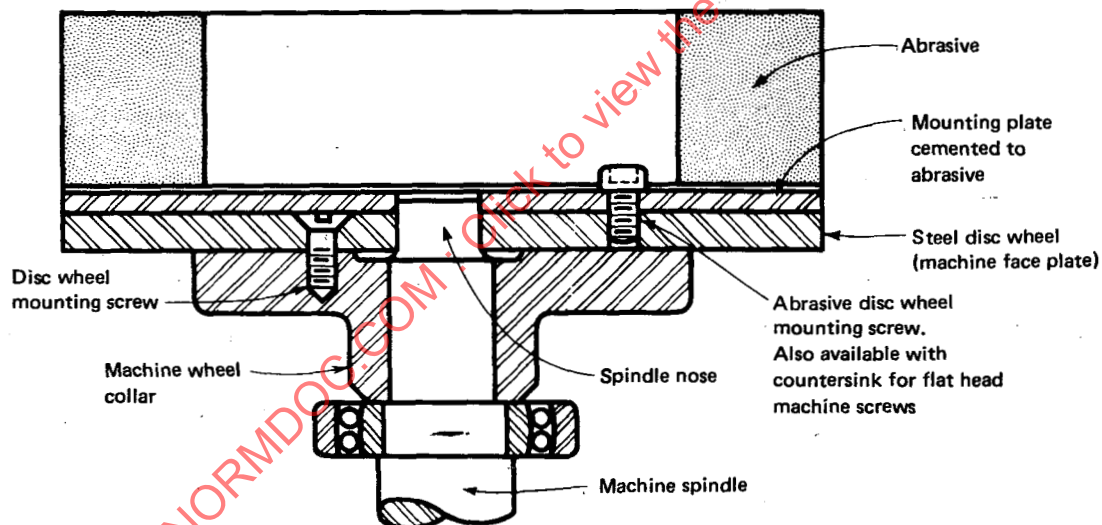
FIG. 6 TYPICAL PLATE TYPE MOUNTING
