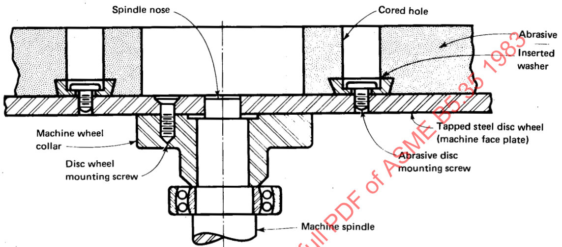
FIG. 2 TYPICAL INSERTED WASHER TYPE MOUNTING
