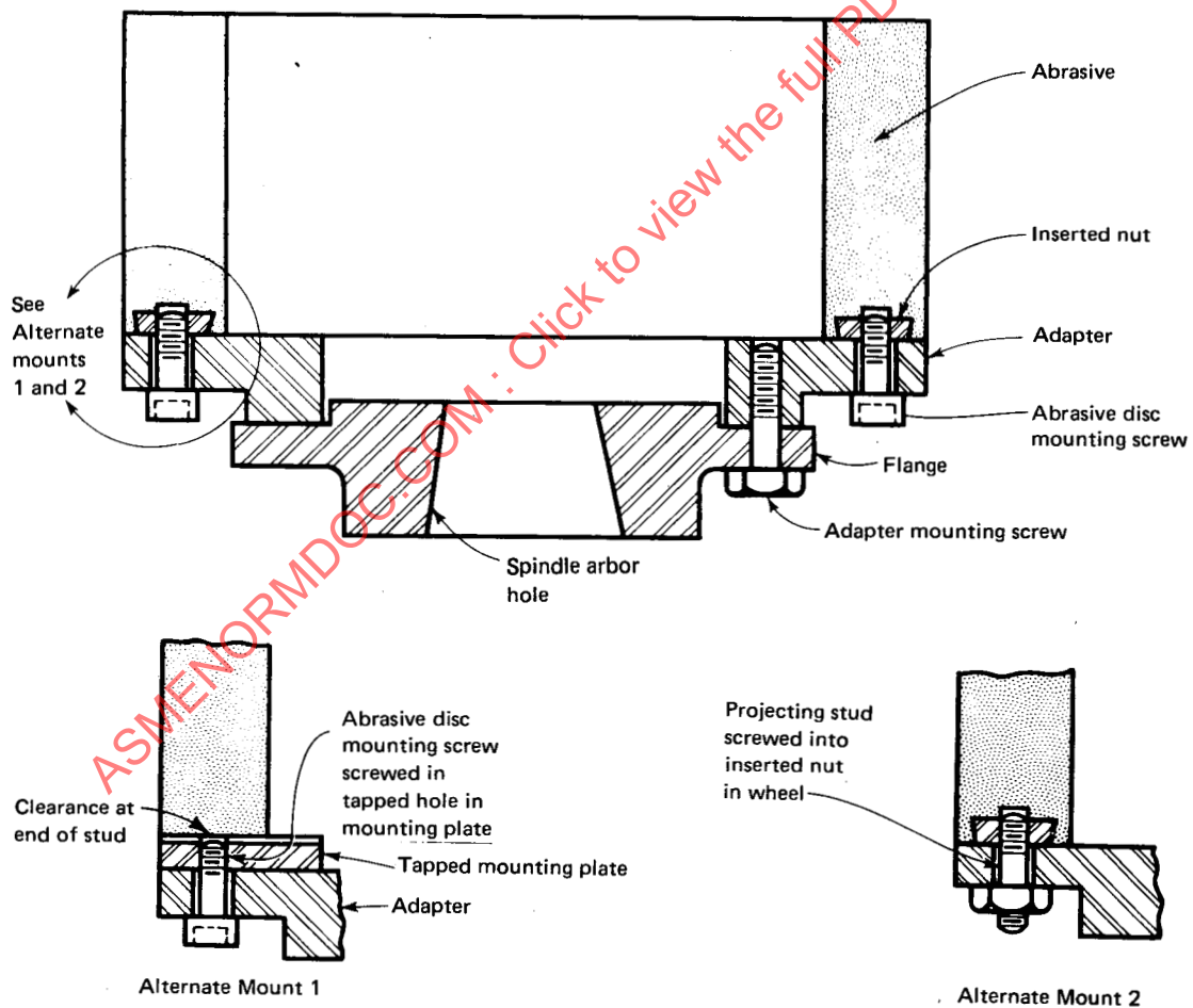
FIG. 5 TYPICAL CYLINDER TYPE MOUNTINGS
