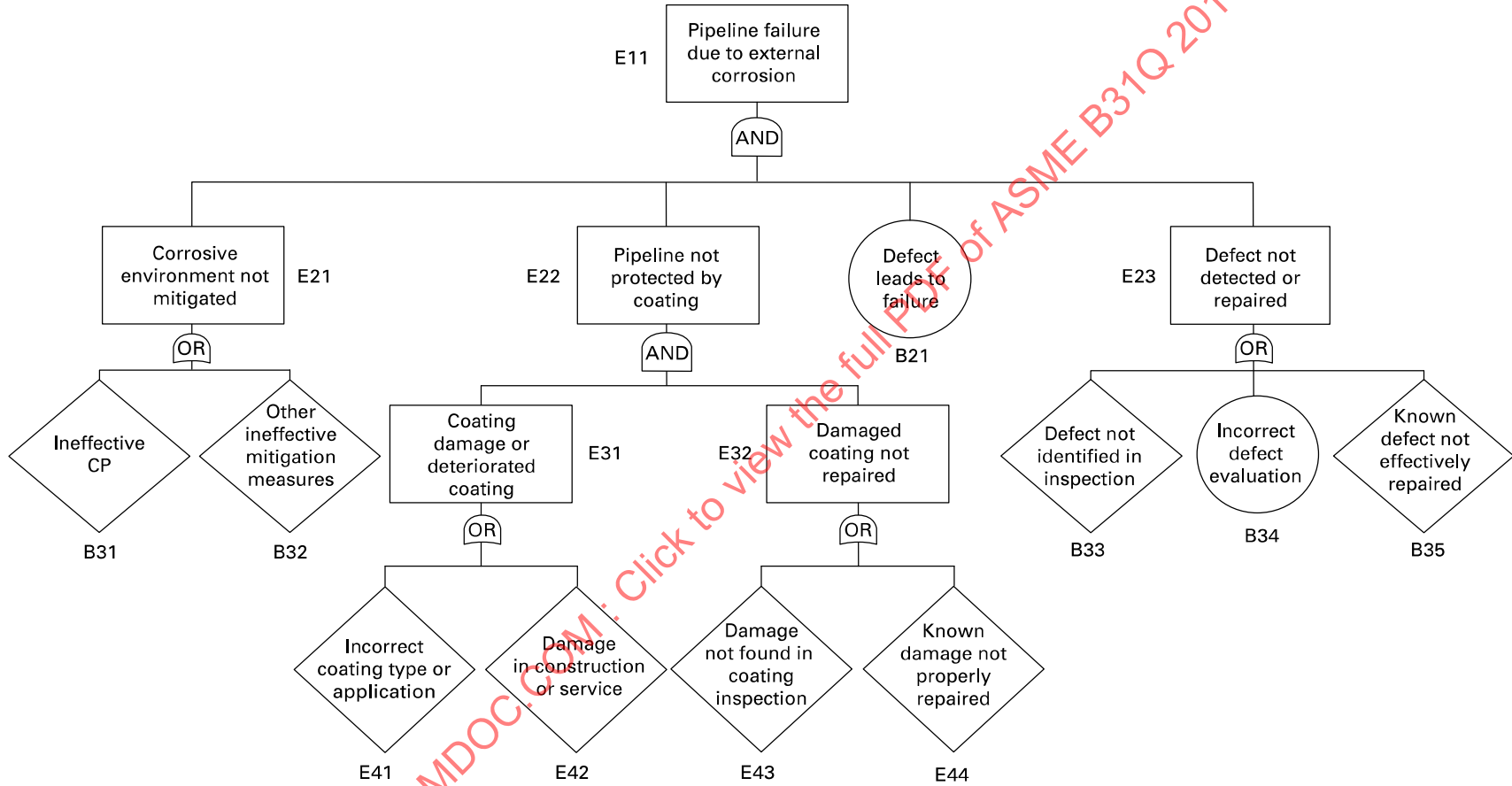
Figure 5.4-1 Fault Tree Example
