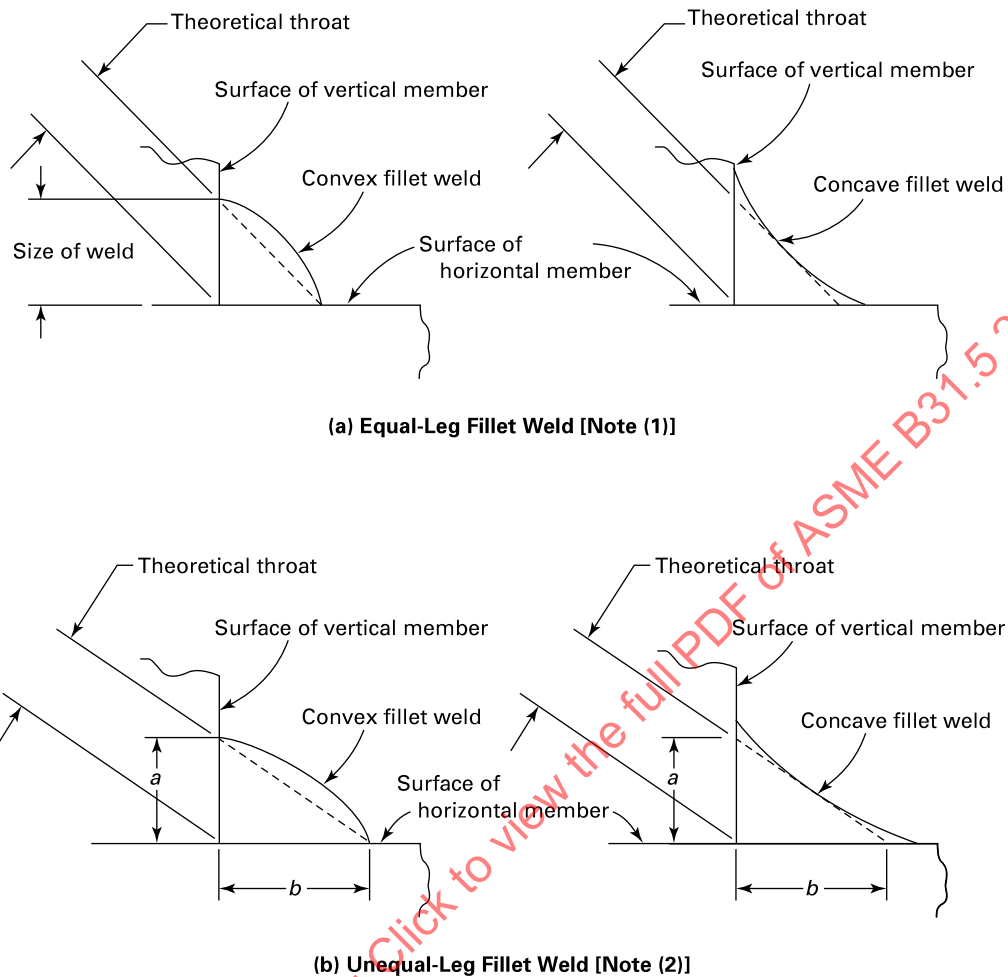
Figure 527.3.3-1 Fillet Weld Size
