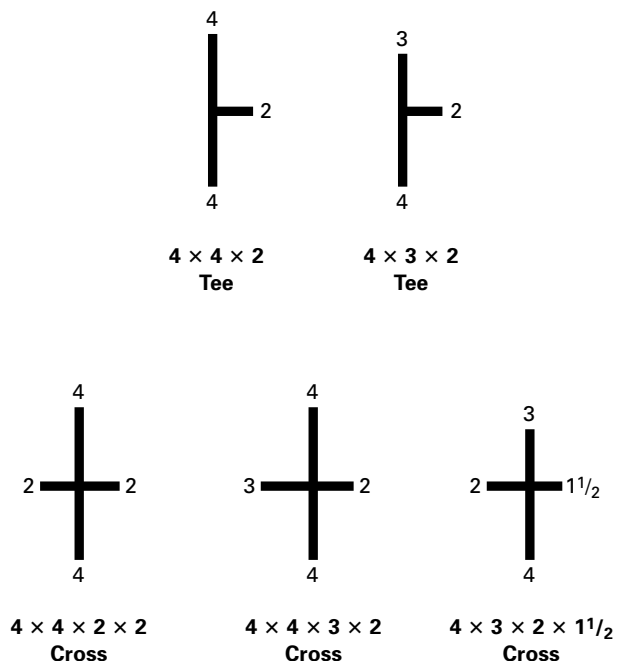
Figure 4.2-1 Identification of Reducing Fittings
